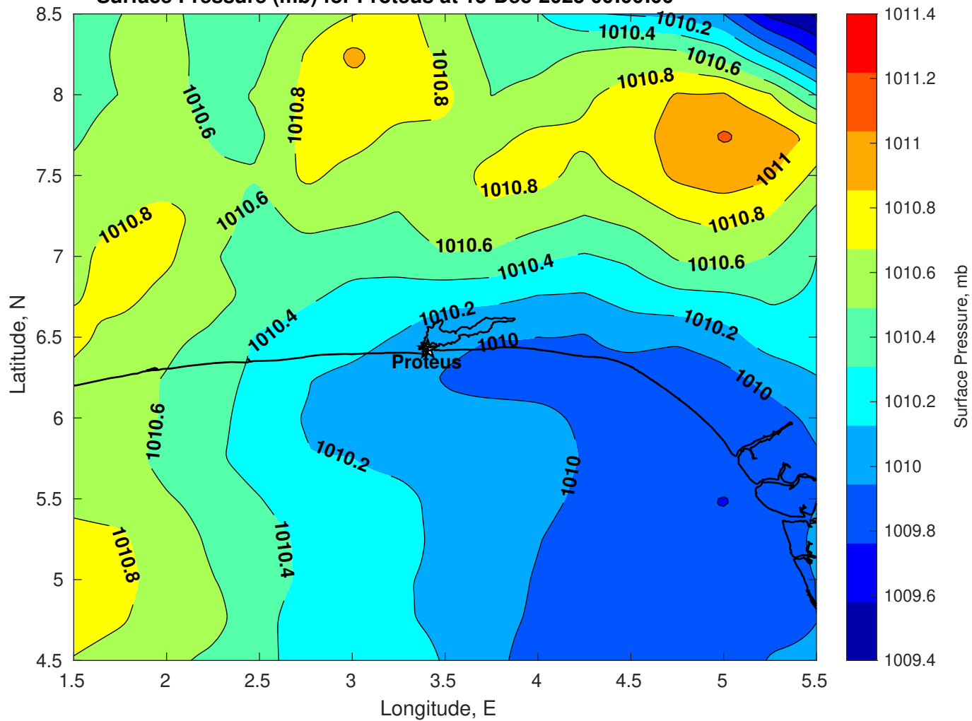
Surface Pressure (mb) for Proteus at 15-Dec-2025 00:00:00
