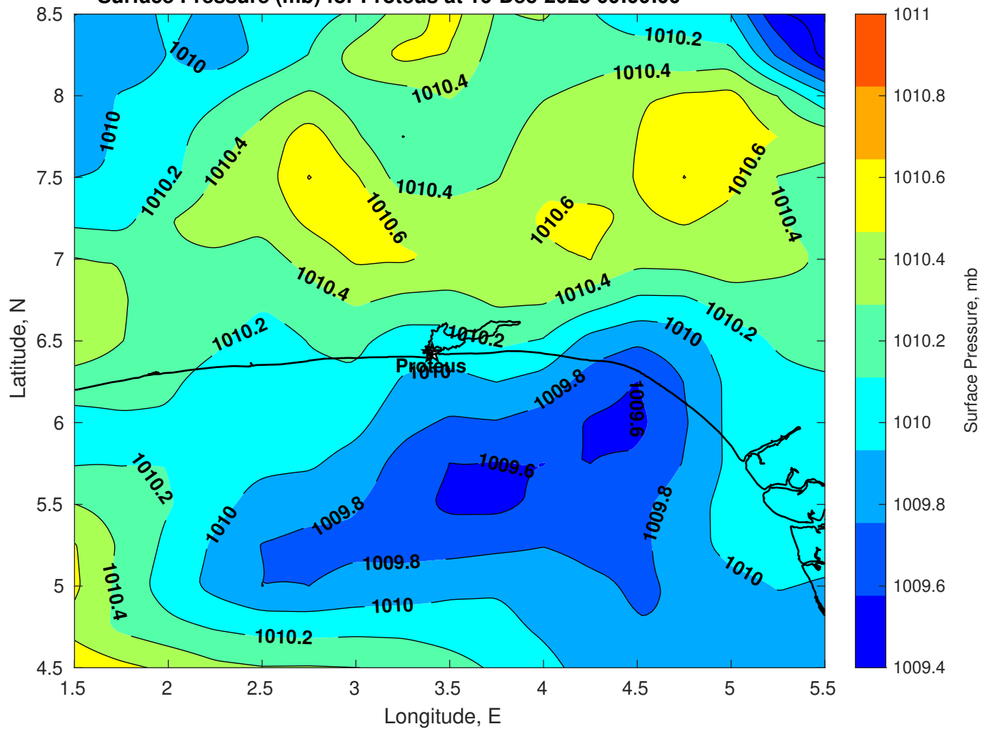
Surface Pressure (mb) for Proteus at 16-Dec-2025 00:00:00
