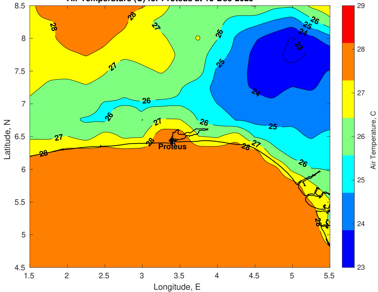
Air Temperature (C) for Proteus at 15-Dec-2025
