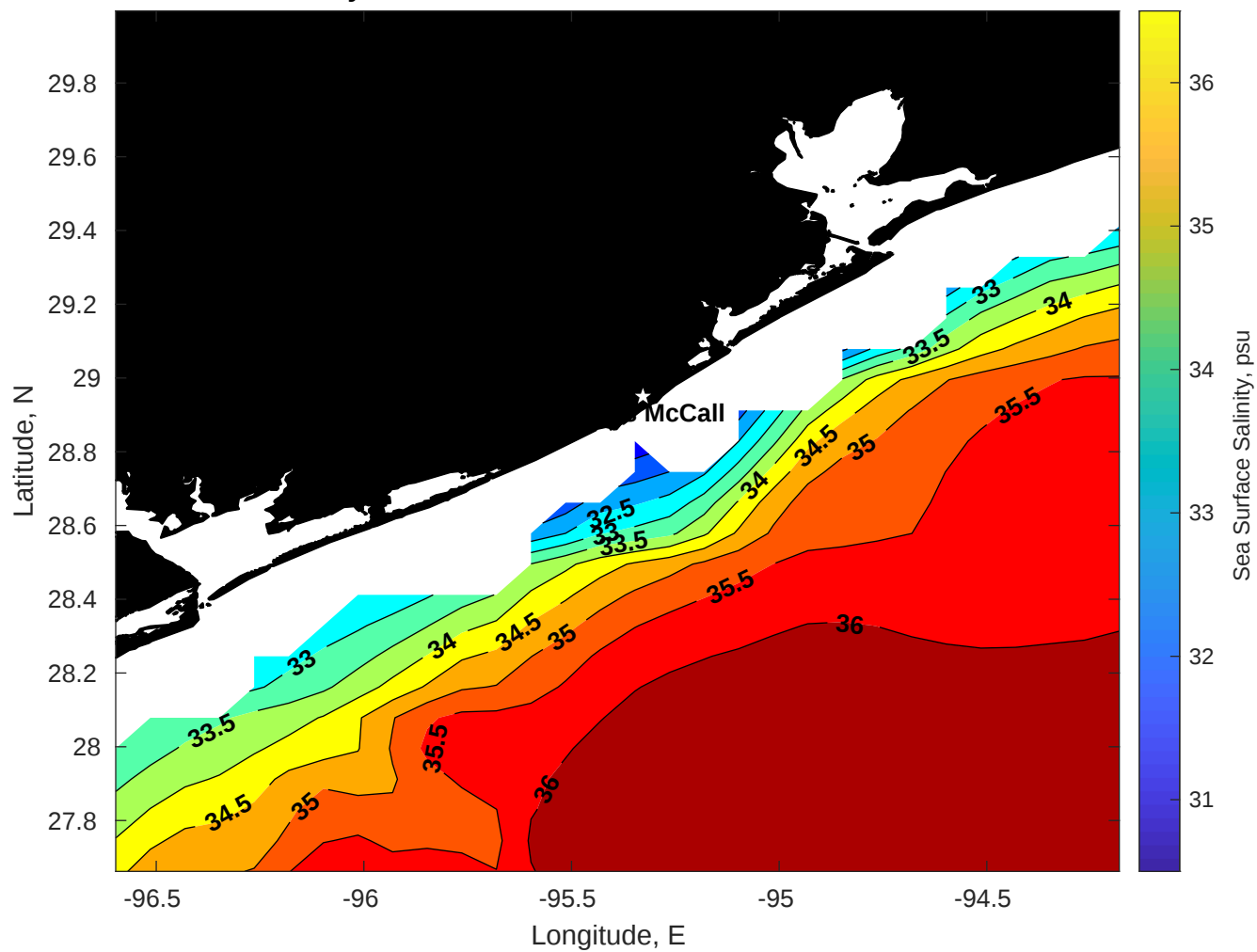
Surface Salinity for Brooks McCall at 15-Dec-2025 00:00:00
