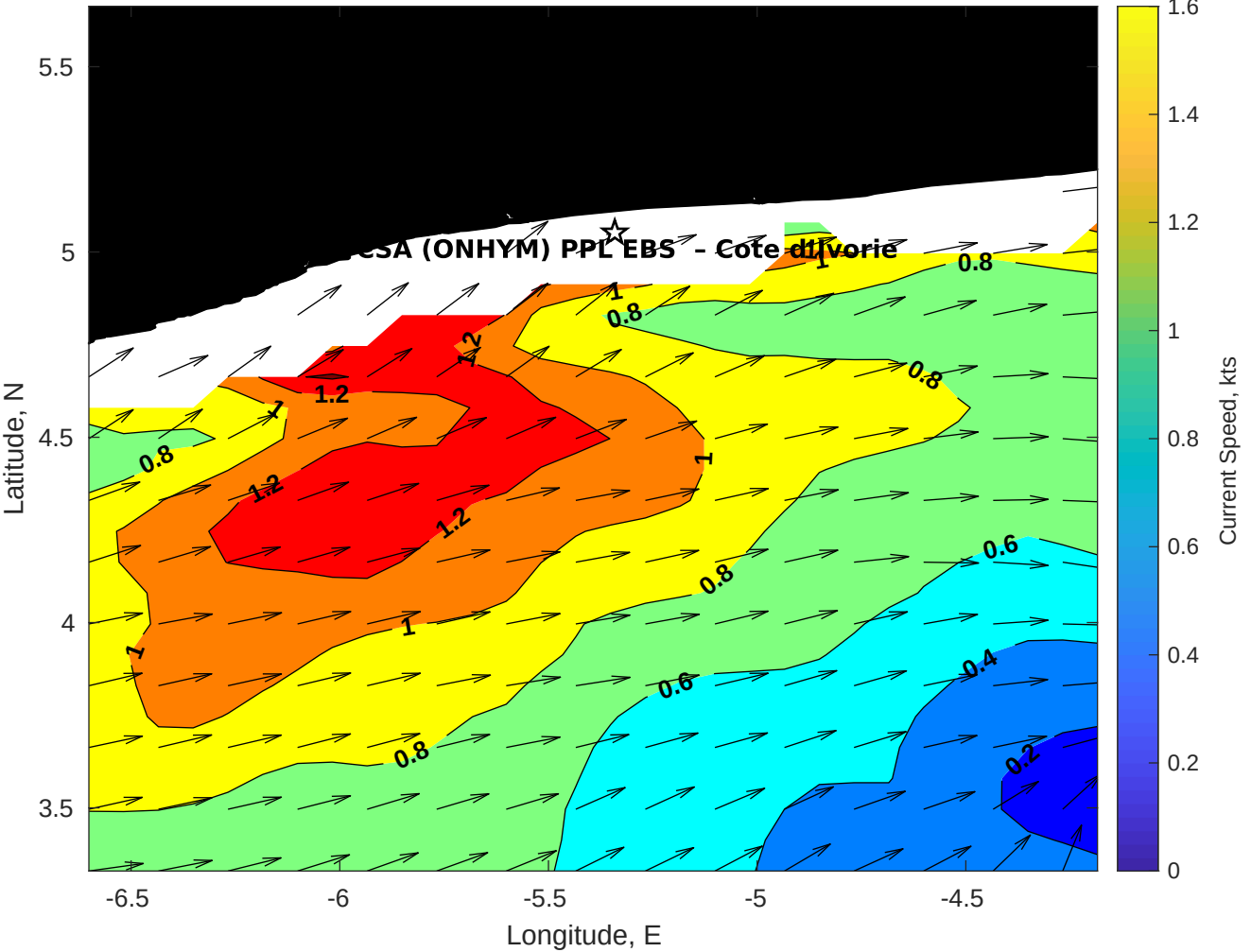
Surface Currents for CSA (ONHYM) PPL EBS - Cote d'Ivoire at 15-Dec-2025 00:00:00
