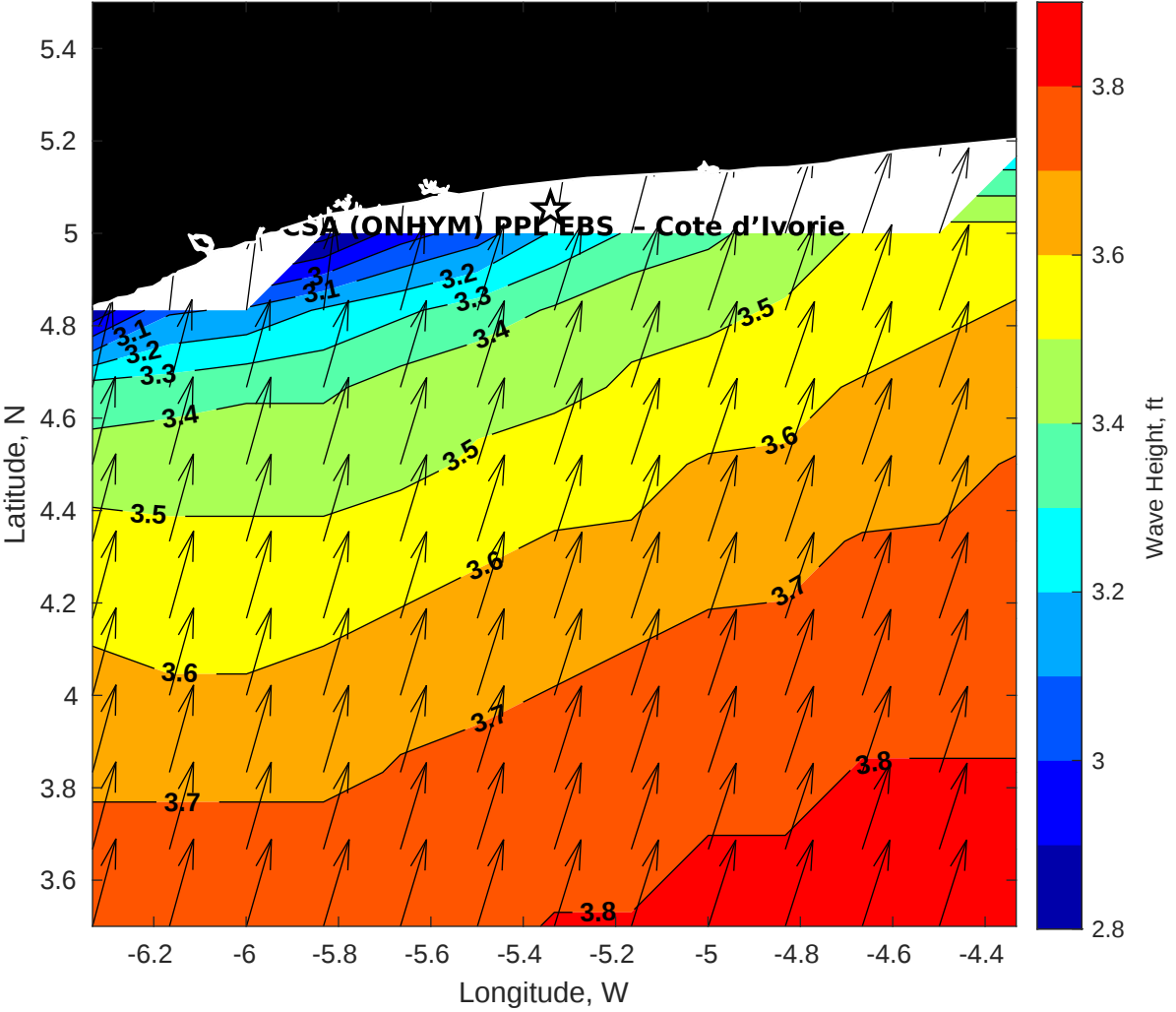
GFS Wave Height (ft) for CSA (ONHYM) PPL EBS - Cote d'Ivoire at 16-Dec-2025 09:00:00
