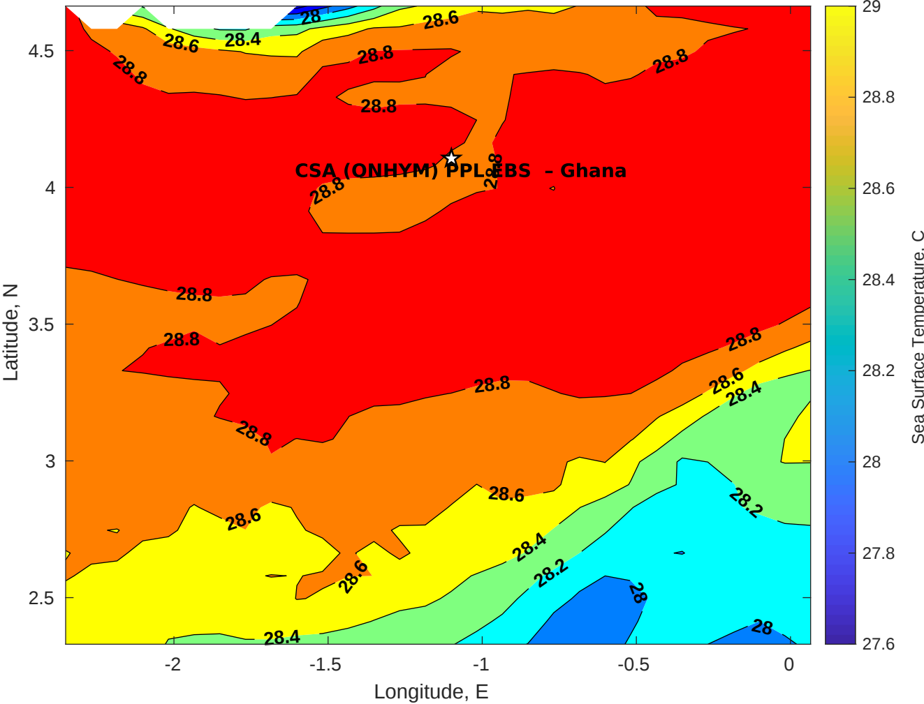
SST for CSA (ONHYM) PPL EBS - Ghana at 15-Dec-2025 00:00:00
