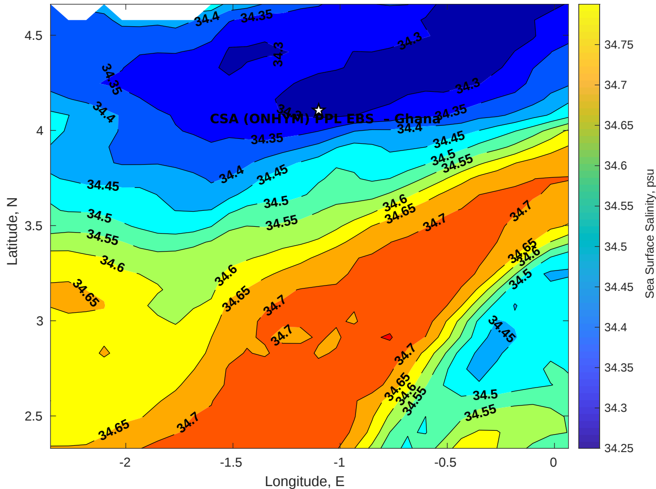
Surface Salinity for CSA (ONHYM) PPL EBS - Ghana at 15-Dec-2025 00:00:00
