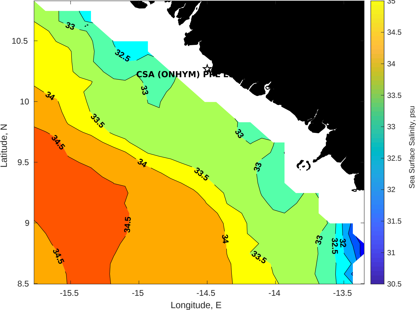
Surface Salinity for CSA (ONHYM) PPL EBS - Guinea at 15-Dec-2025 00:00:00
