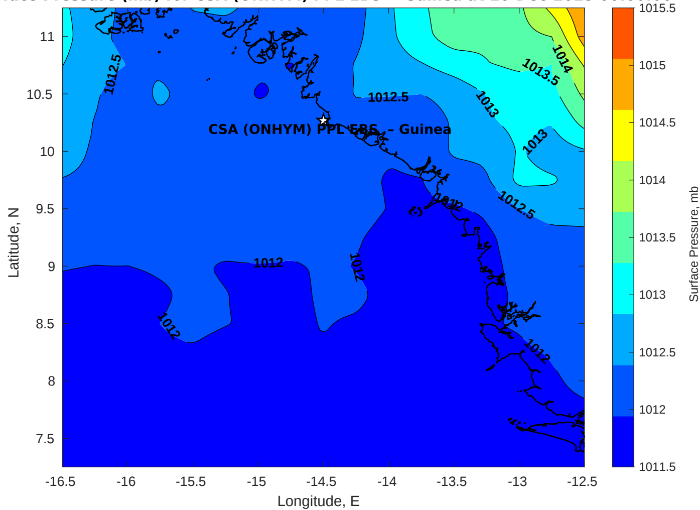
Surface Pressure (mb) for CSA (ONHYM) PPL EBS - Guinea at 16-Dec-2025 00:00:00
