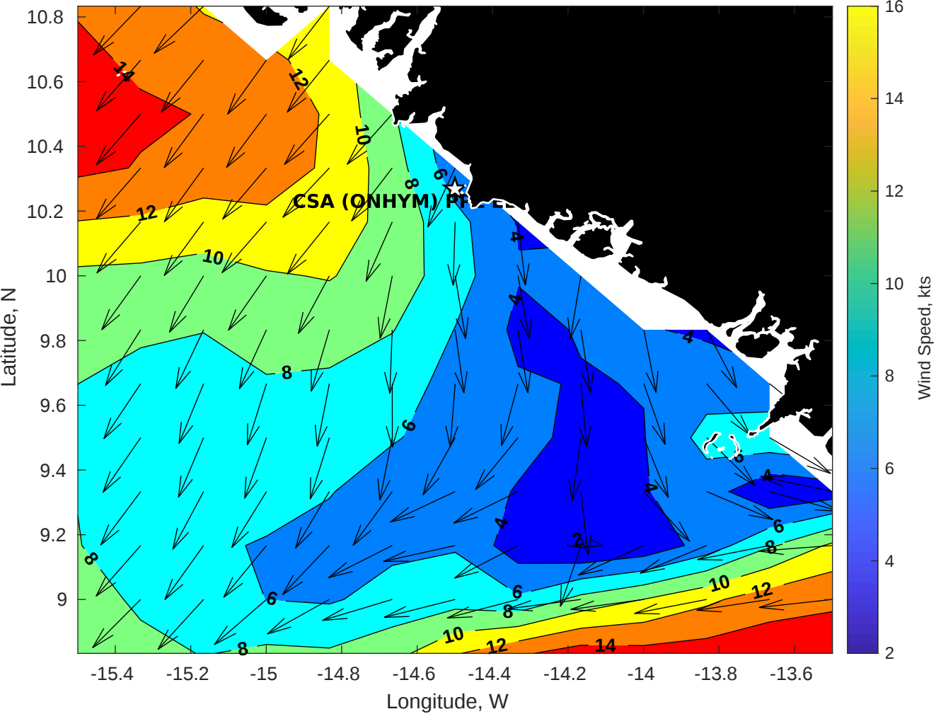
GFS Winds (kts) for CSA (ONHYM) PPL EBS - Guinea at 16-Dec-2025 09:00:00
