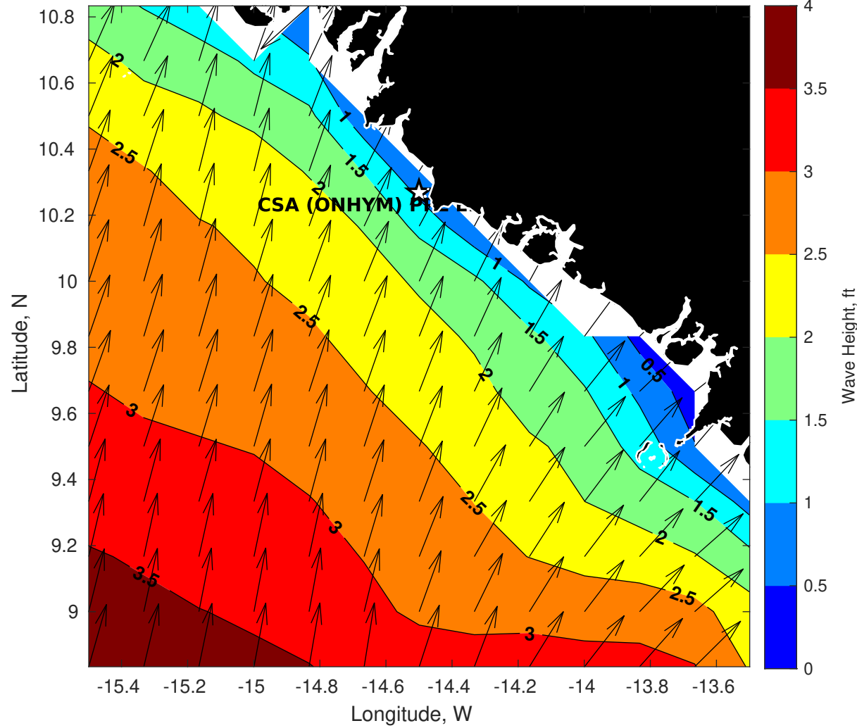
GFS Wave Height (ft) for CSA (ONHYM) PPL EBS - Guinea at 16-Dec-2025 09:00:00
