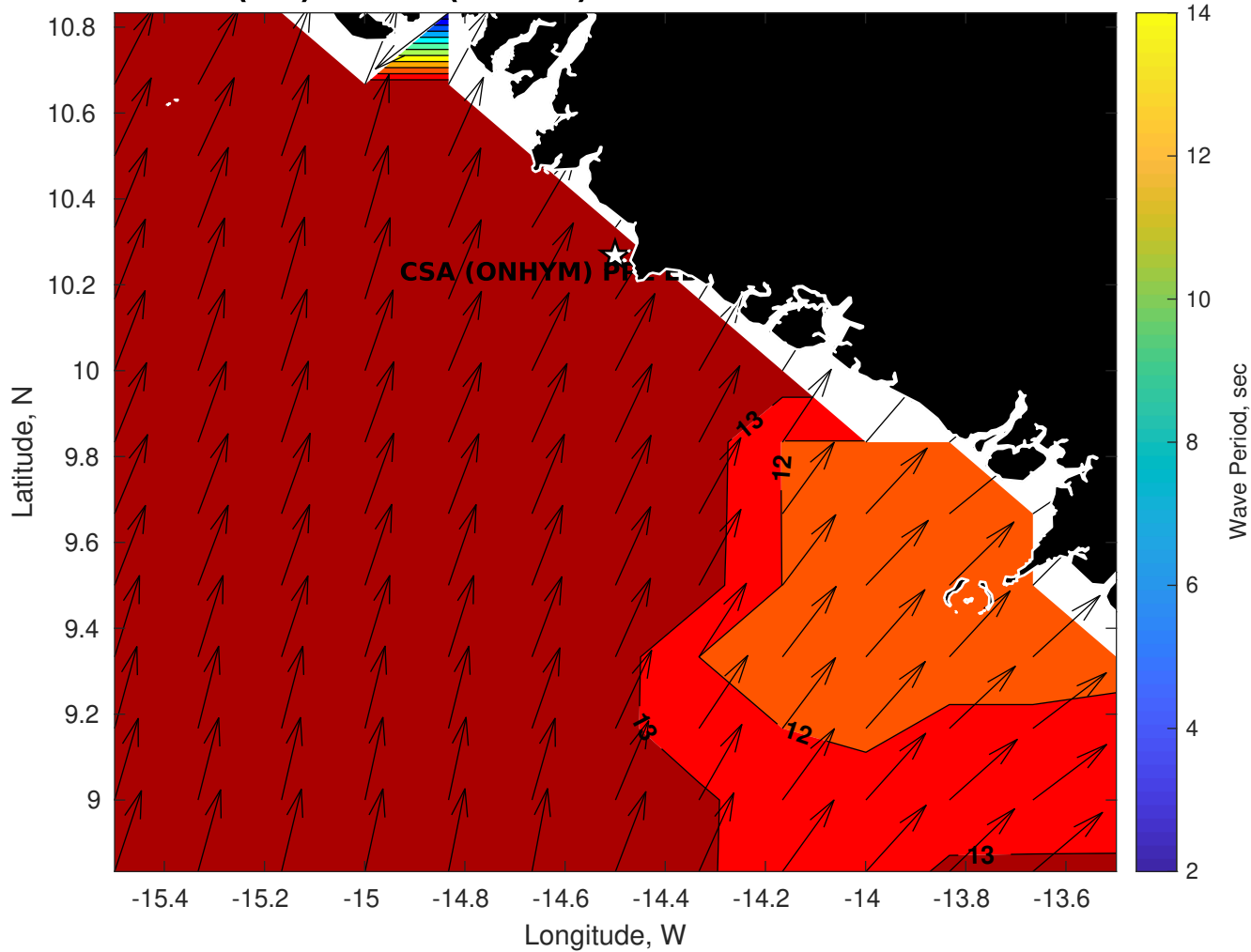
GFS Wave Period (sec) for CSA (ONHYM) PPL EBS - Guinea at 16-Dec-2025 09:00:00
