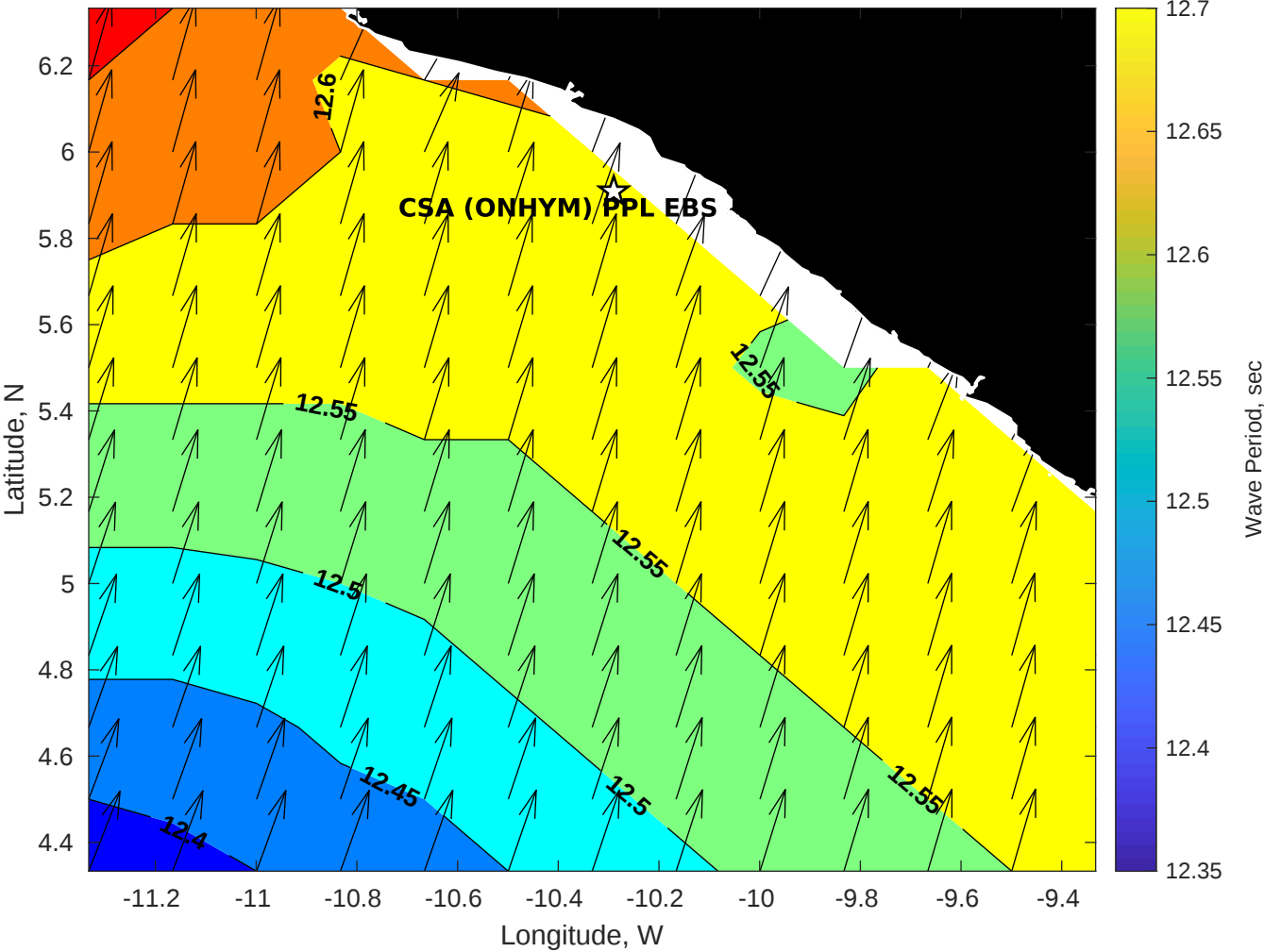
GFS Wave Period (sec) for CSA (ONHYM) PPL EBS - Liberia at 16-Dec-2025 09:00:00
