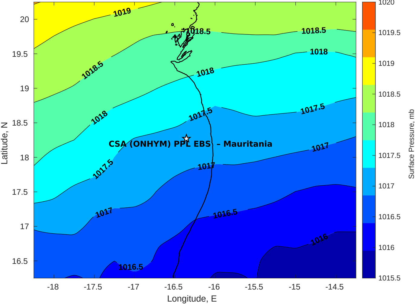
Surface Pressure (mb) for CSA (ONHYM) PPL EBS - Mauritania at 17-Dec-2025 00:00:00
