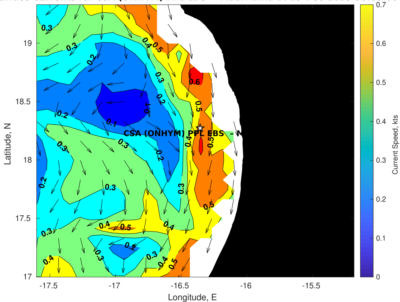
Surface Currents for CSA (ONHYM) PPL EBS - Mauritania at 15-Dec-2025 00:00:00
