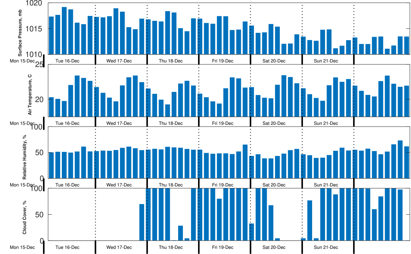
Met Forecast for CSA (ONHYM) PPL EBS - Mauritania from 16-Dec-2025 00:00:00 to 23-Dec-2025 00:00:00
