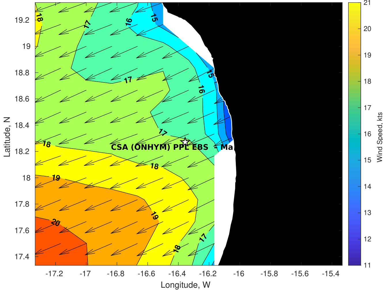
GFS Winds (kts) for CSA (ONHYM) PPL EBS - Mauritania at 16-Dec-2025 09:00:00
