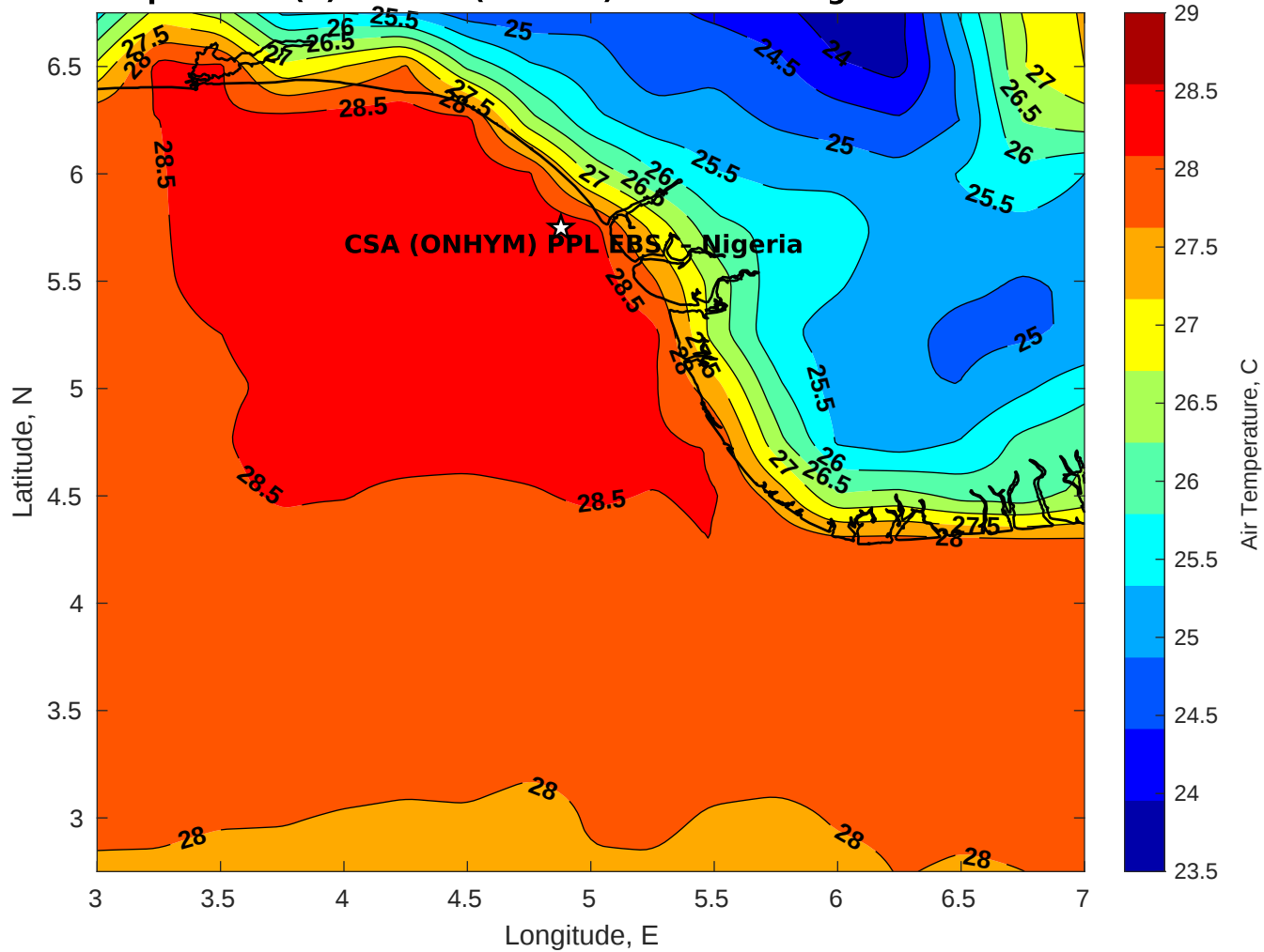
Air Temperature (C) for CSA (ONHYM) PPL EBS - Nigeria at 16-Dec-2025
