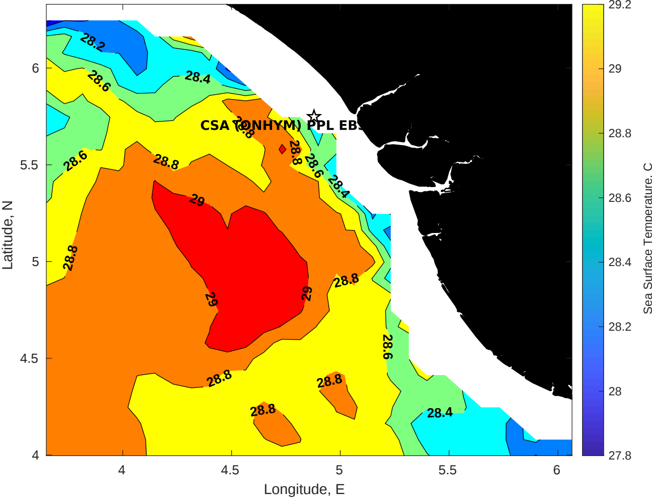
SST for CSA (ONHYM) PPL EBS - Nigeria at 15-Dec-2025 00:00:00
