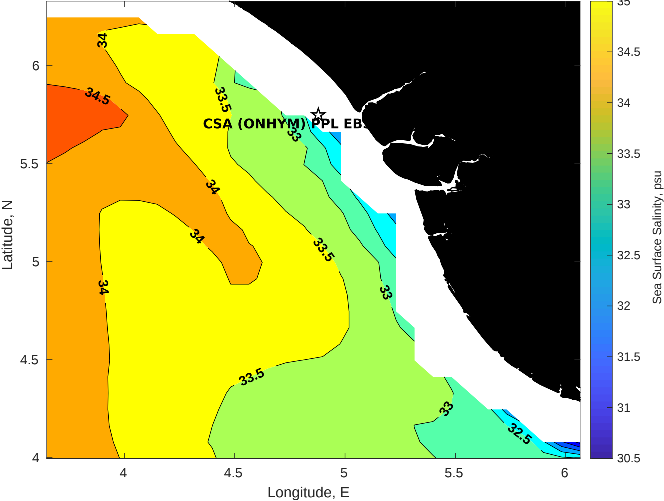
Surface Salinity for CSA (ONHYM) PPL EBS - Nigeria at 15-Dec-2025 00:00:00
