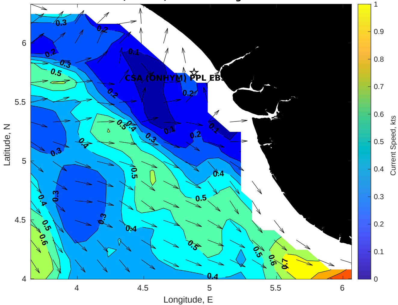
Surface Currents for CSA (ONHYM) PPL EBS - Nigeria at 15-Dec-2025 00:00:00
