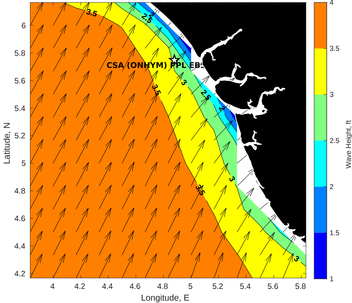
GFS Wave Height (ft) for CSA (ONHYM) PPL EBS - Nigeria at 16-Dec-2025 09:00:00
