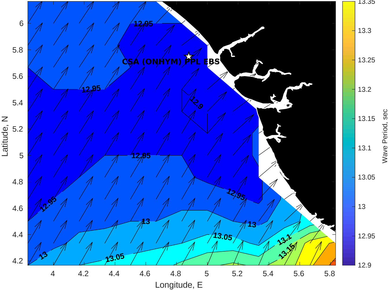
GFS Wave Period (sec) for CSA (ONHYM) PPL EBS - Nigeria at 16-Dec-2025 09:00:00
