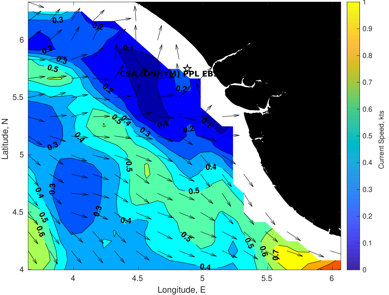
Surface Currents for CSA (ONHYM) PPL EBS - Nigeria at 15-Dec-2025 00:00:00
