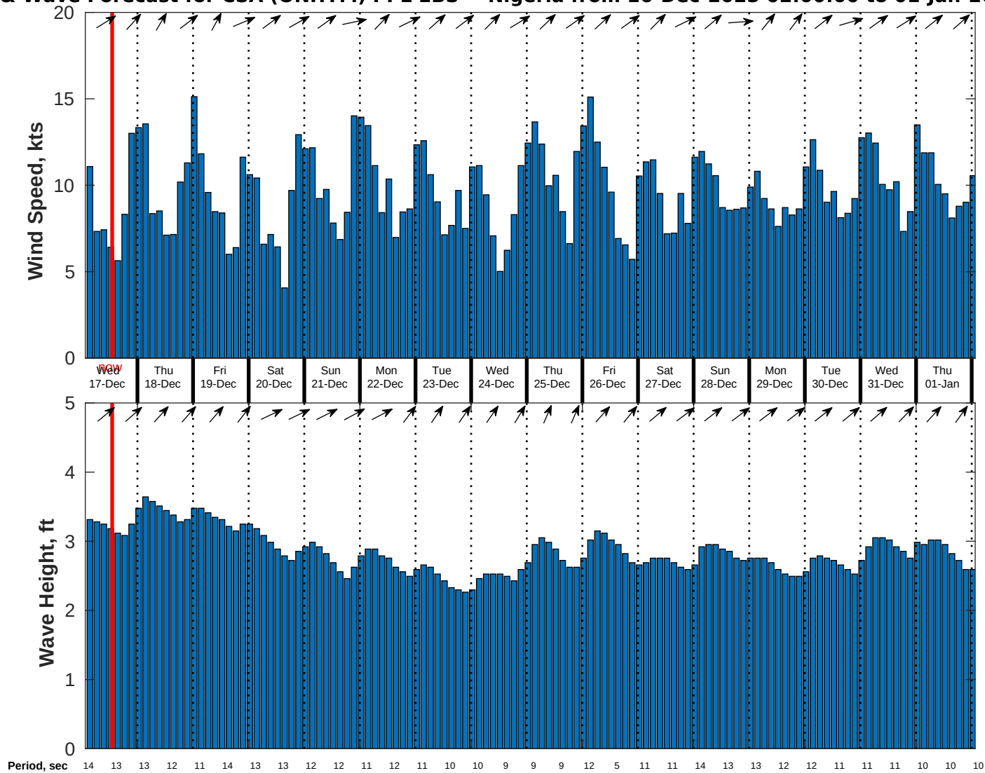
Wind & Wave Forecast for CSA (ONHYM) PPL EBS - Nigeria from 16-Dec-2025 02:00:00 to 01-Jan-2026 02:00:00
