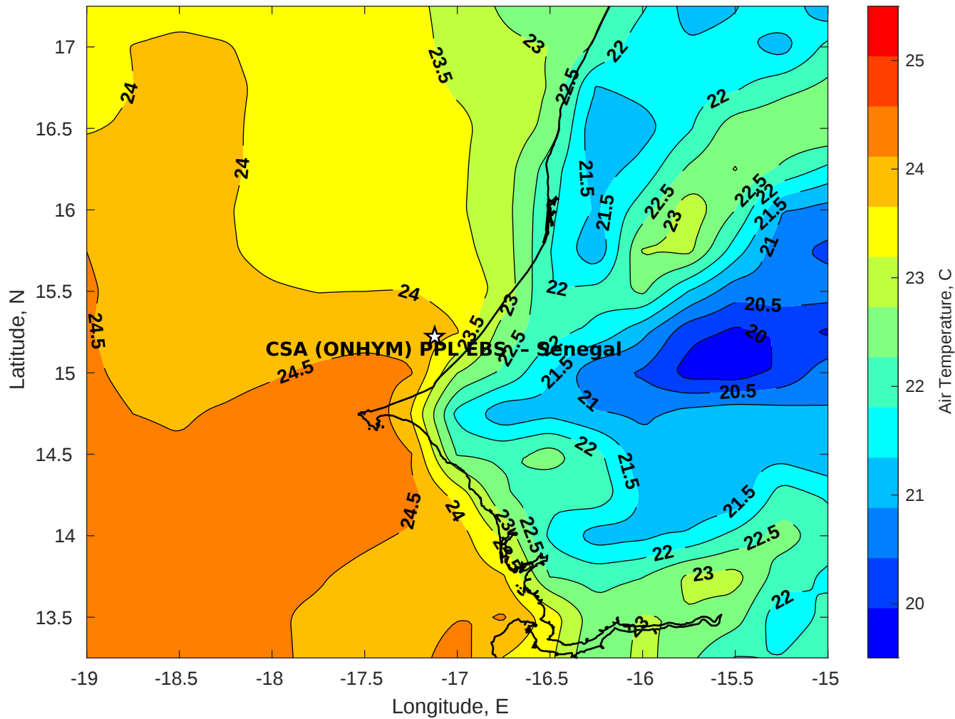
Air Temperature (C) for CSA (ONHYM) PPL EBS - Senegal at 16-Dec-2025
