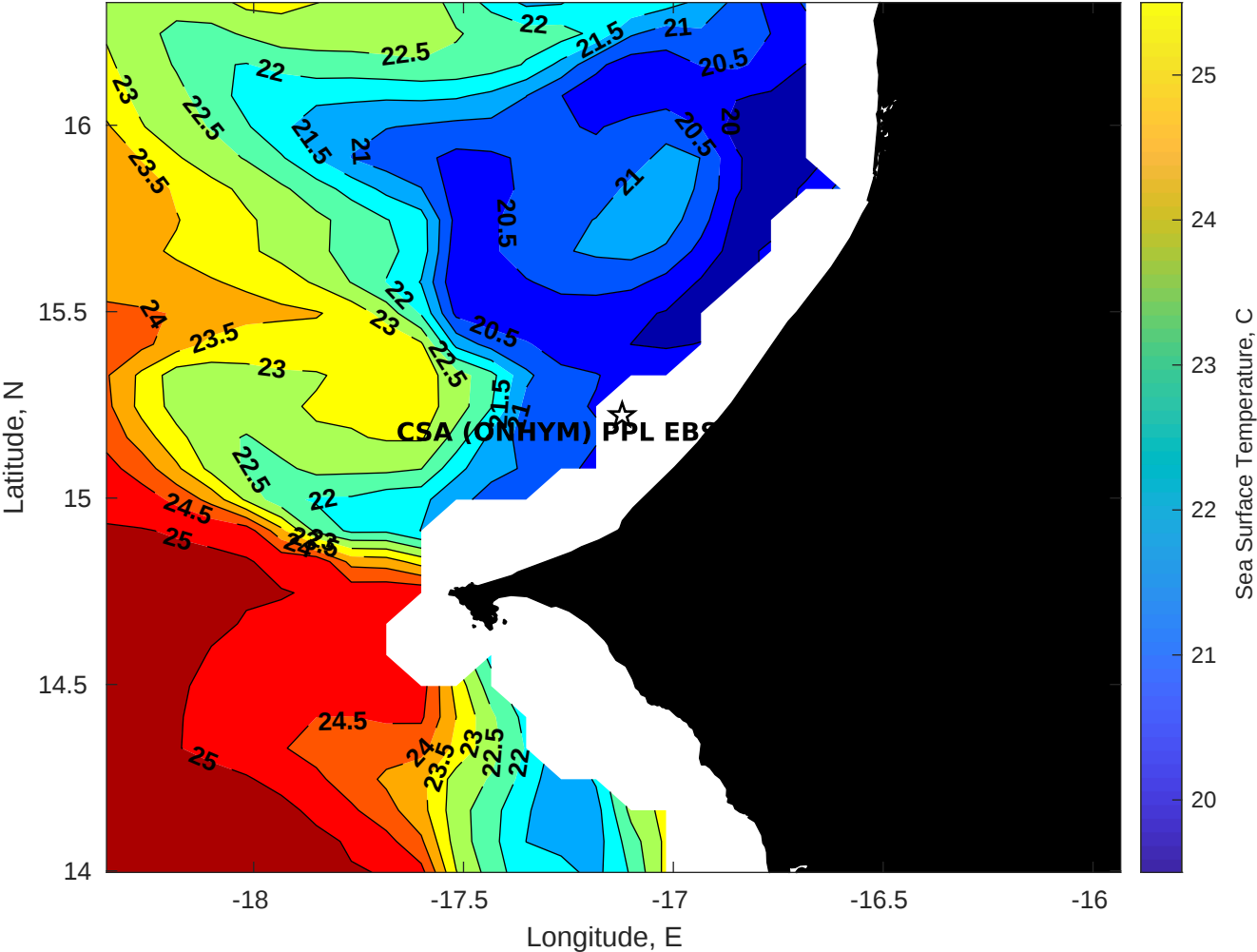
SST for CSA (ONHYM) PPL EBS - Senegal at 15-Dec-2025 00:00:00
