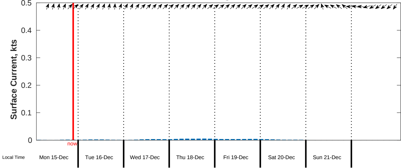
Surface Current Forecast for CSA (ONHYM) PPL EBS - Senegal from 15-Dec-2025 00:00:00 to 23-Dec-2025 00:00:00
