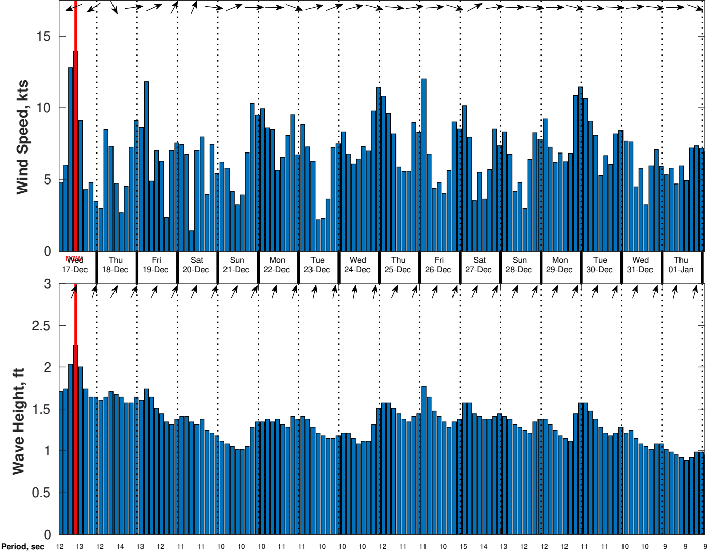
Wind & Wave Forecast for CSA (ONHYM) PPL EBS - Sierra Leone from 16-Dec-2025 01:00:00 to 01-Jan-2026 01:00:00
