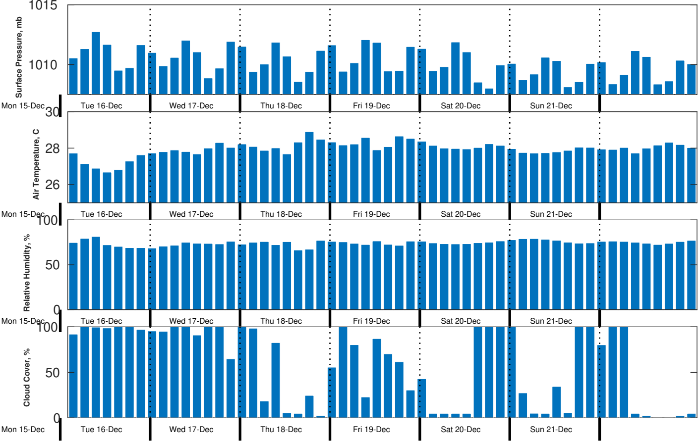
Met Forecast for CSA (ONHYM) PPL EBS - Sierra Leone from 16-Dec-2025 00:00:00 to 23-Dec-2025 00:00:00
