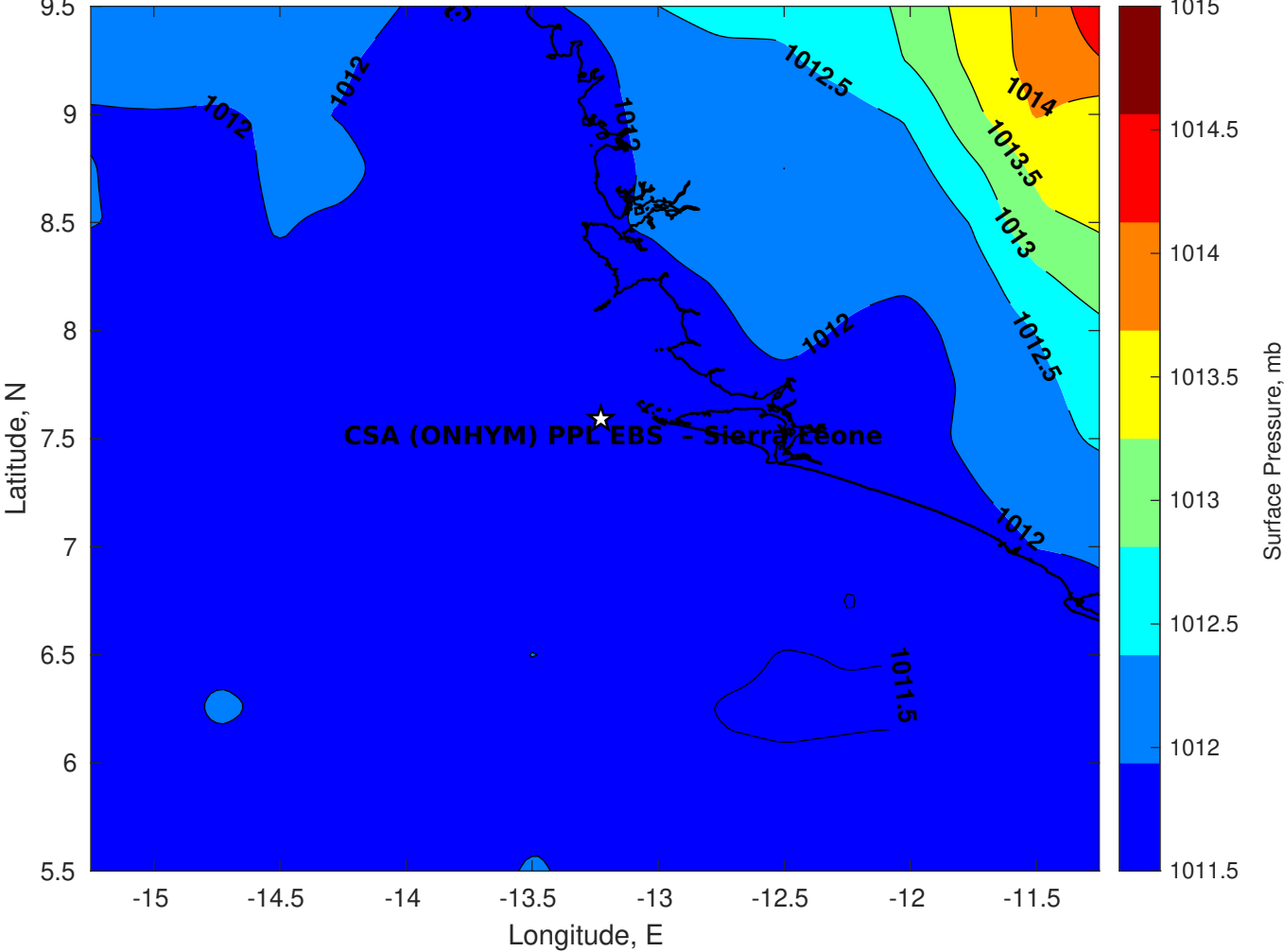
Surface Pressure (mb) for CSA (ONHYM) PPL EBS - Sierra Leone at 16-Dec-2025 00:00:00
