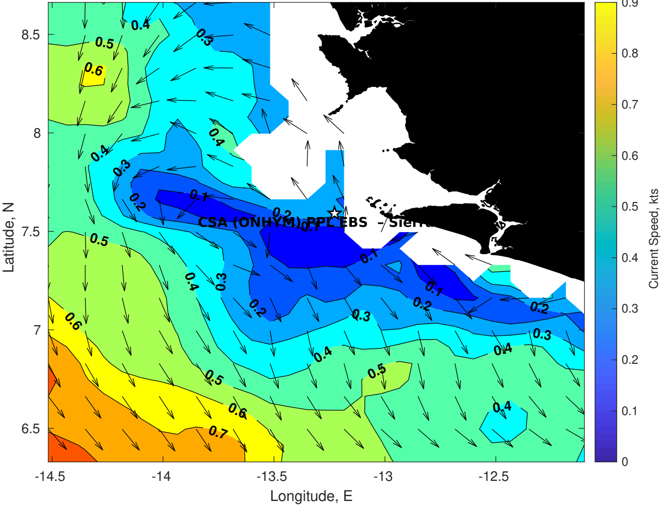
Surface Currents for CSA (ONHYM) PPL EBS - Sierra Leone at 15-Dec-2025 00:00:00
