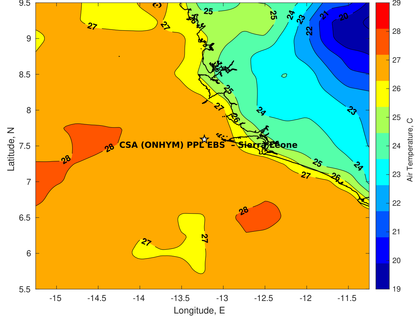
Air Temperature (C) for CSA (ONHYM) PPL EBS - Sierra Leone at 16-Dec-2025
