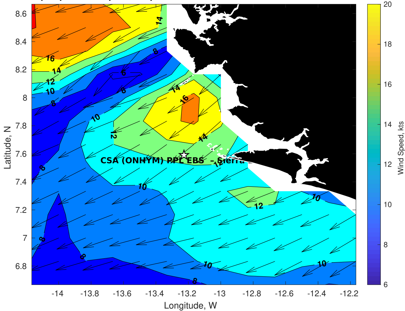
GFS Winds (kts) for CSA (ONHYM) PPL EBS - Sierra Leone at 16-Dec-2025 09:00:00
