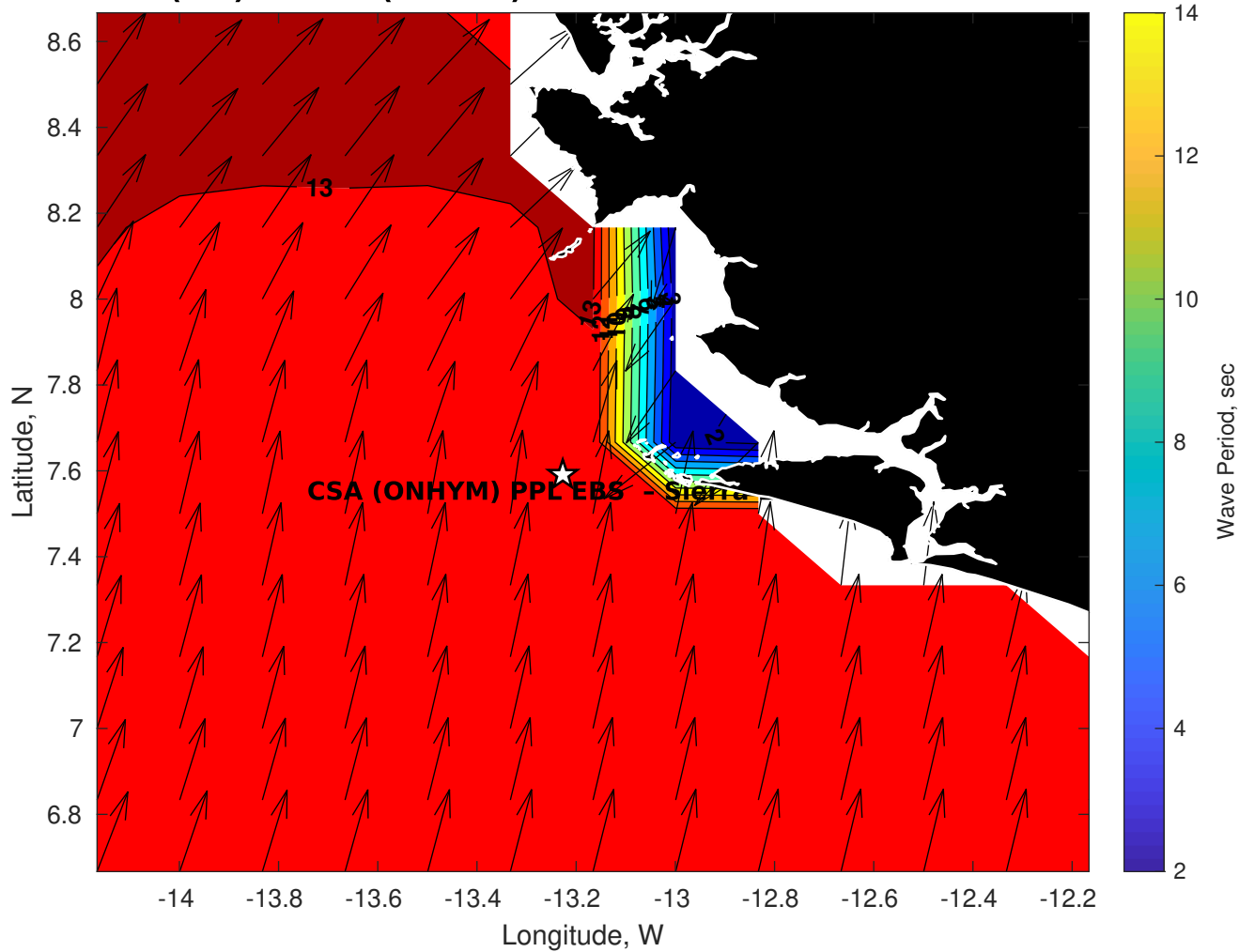
GFS Wave Period (sec) for CSA (ONHYM) PPL EBS - Sierra Leone at 16-Dec-2025 09:00:00
