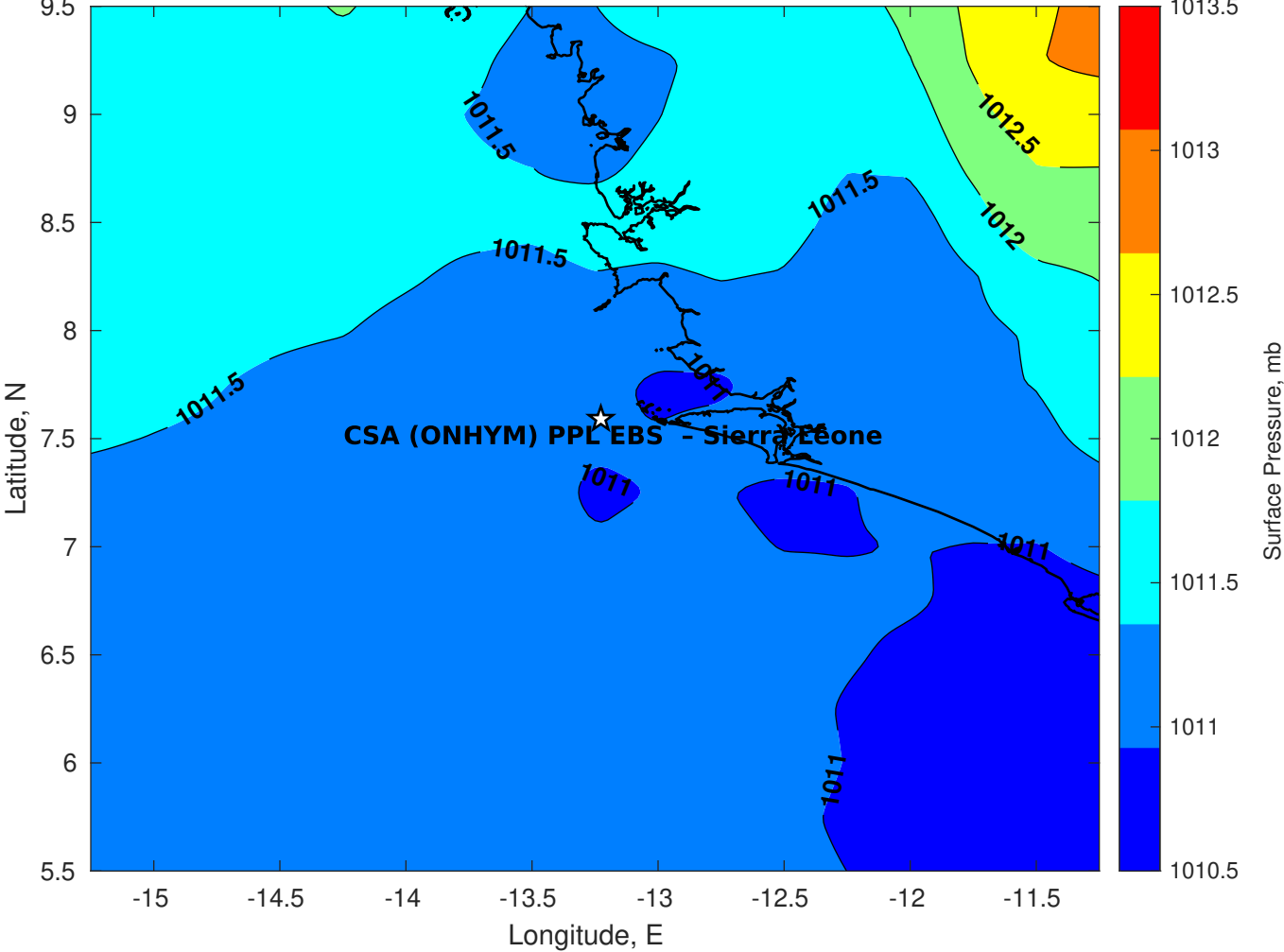
Surface Pressure (mb) for CSA (ONHYM) PPL EBS - Sierra Leone at 17-Dec-2025 00:00:00
