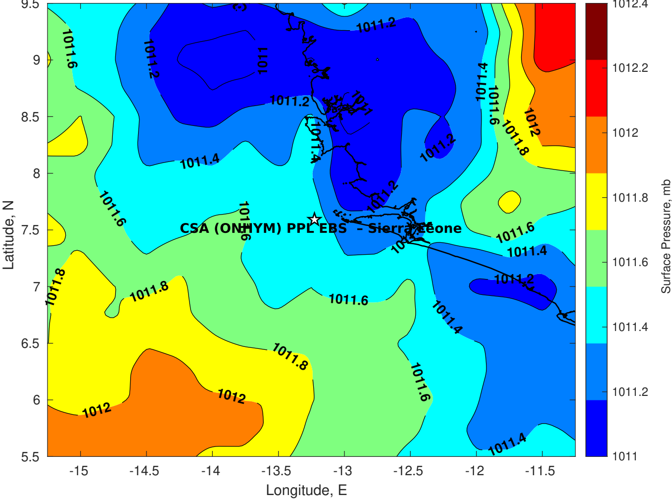
Surface Pressure (mb) for CSA (ONHYM) PPL EBS - Sierra Leone at 18-Dec-2025 00:00:00
