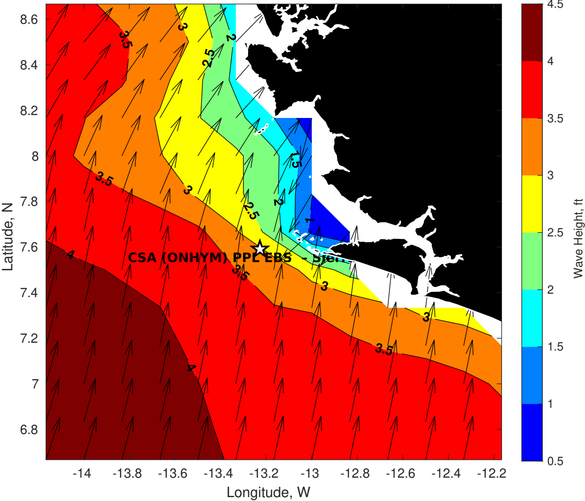
GFS Wave Height (ft) for CSA (ONHYM) PPL EBS - Sierra Leone at 16-Dec-2025 09:00:00
