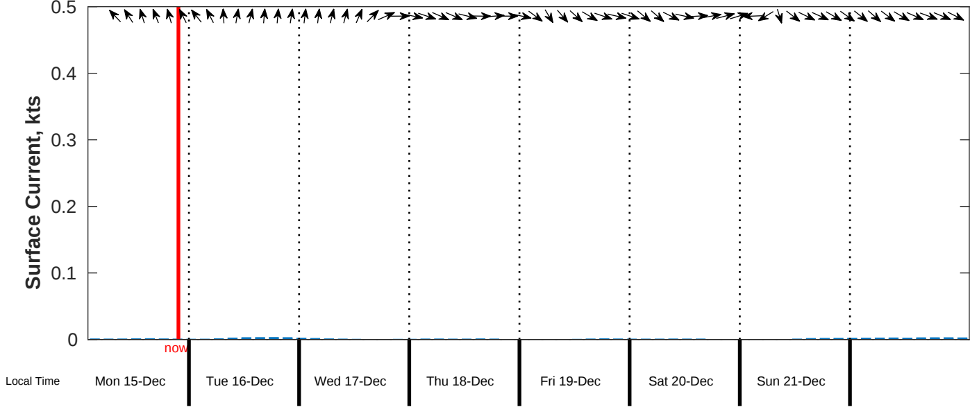
Surface Current Forecast for CSA (ONHYM) PPL EBS - Sierra Leone from 15-Dec-2025 00:00:00 to 23-Dec-2025 00:00:00
