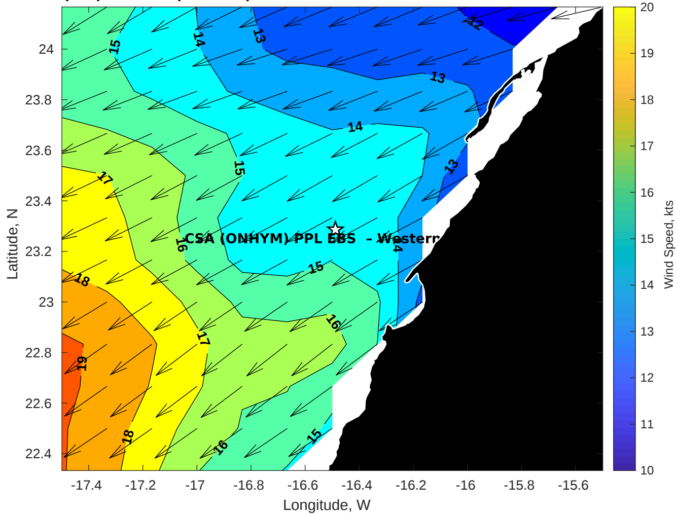
GFS Winds (kts) for CSA (ONHYM) PPL EBS - Western Sahara at 16-Dec-2025 09:00:00
