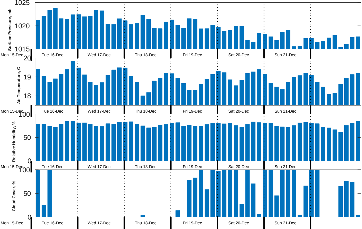
Met Forecast for CSA (ONHYM) PPL EBS - Western Sahara from 16-Dec-2025 00:00:00 to 23-Dec-2025 00:00:00
