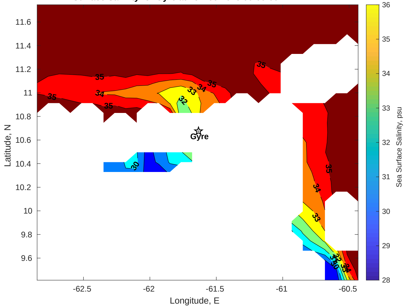
Surface Salinity for Gyre at 15-Dec-2025 00:00:00
