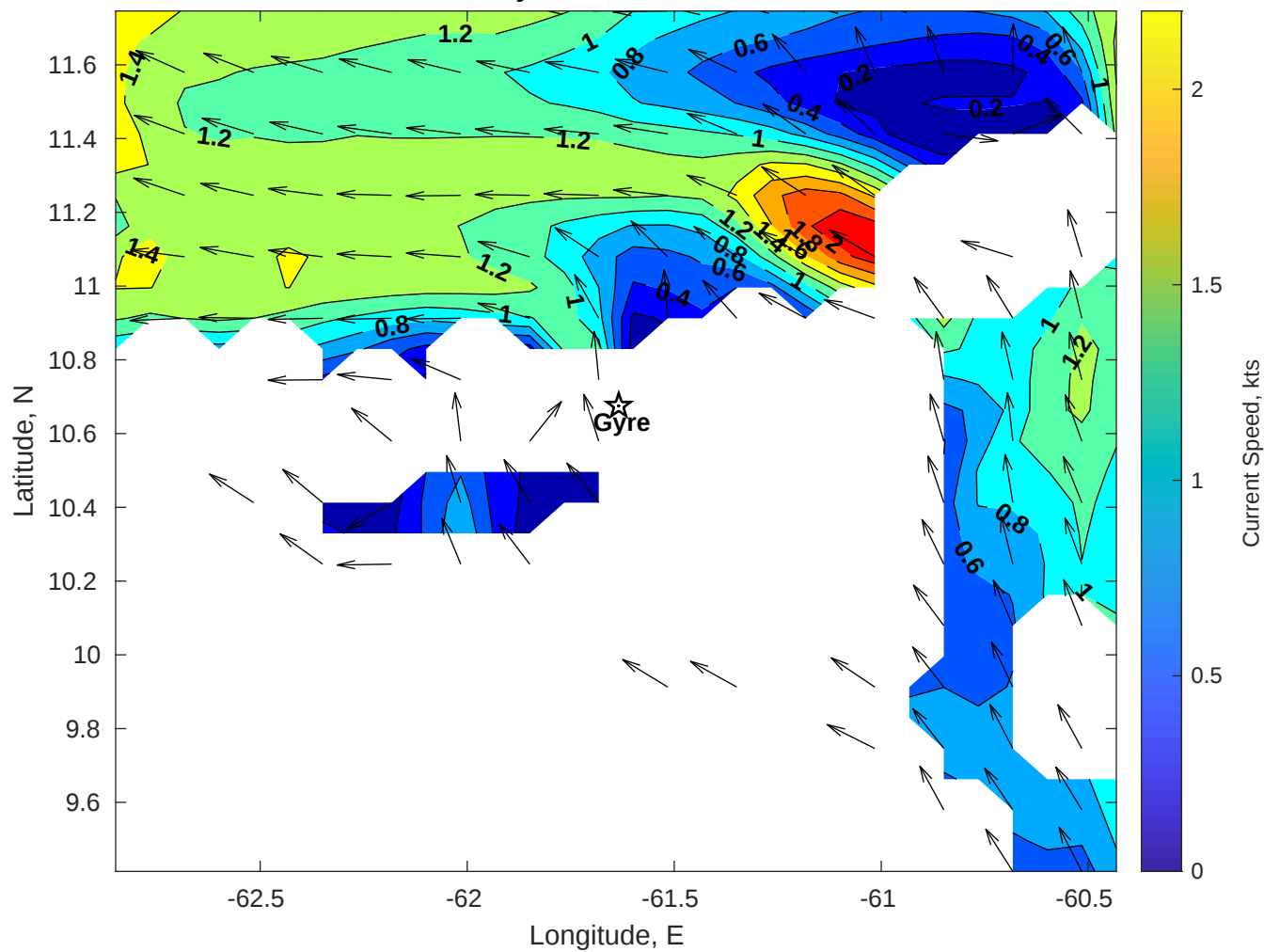
Surface Currents for Gyre at 15-Dec-2025 00:00:00
