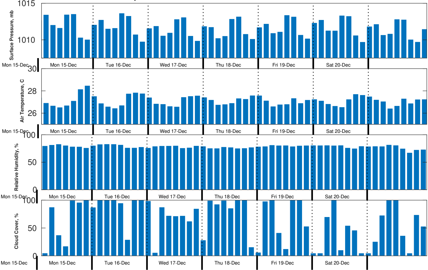
Met Forecast for Gyre from 15-Dec-2025 20:00:00 to 22-Dec-2025 20:00:00
