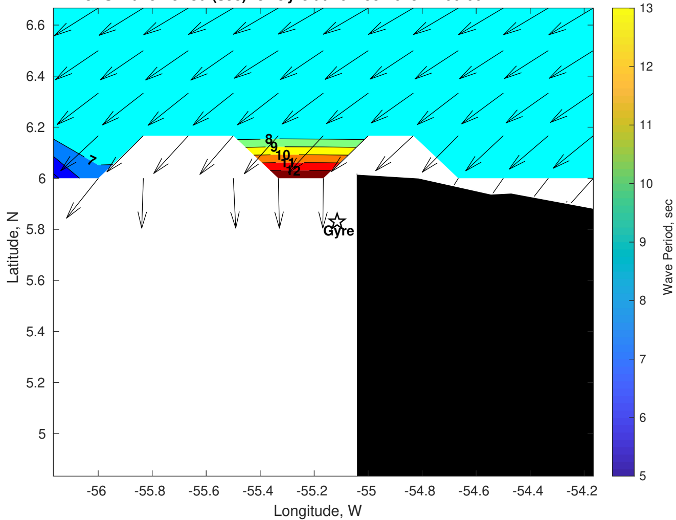
GFS Wave Period (sec) for Gyre at 10-Dec-2025 21:00:00
