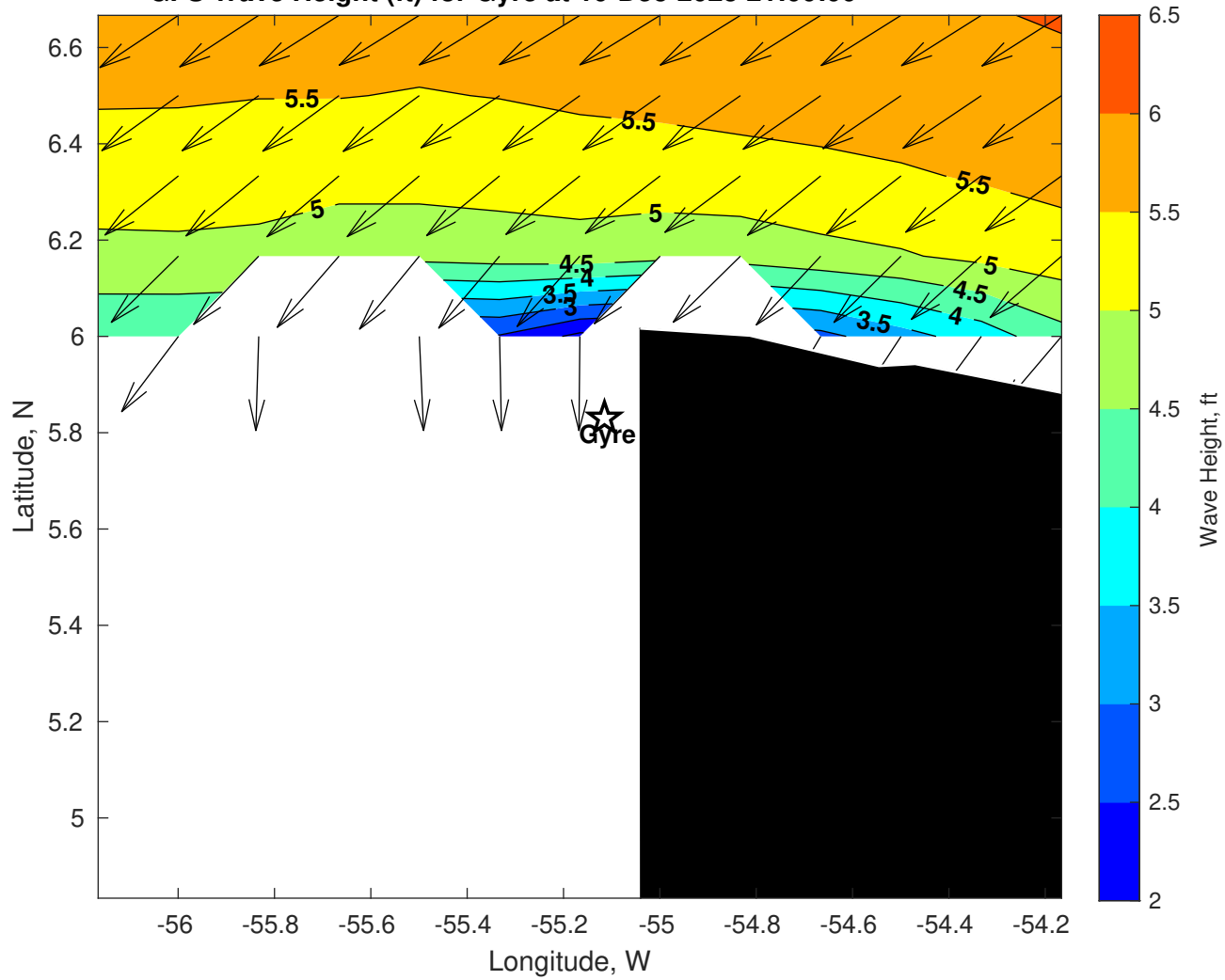
GFS Wave Height (ft) for Gyre at 10-Dec-2025 21:00:00
