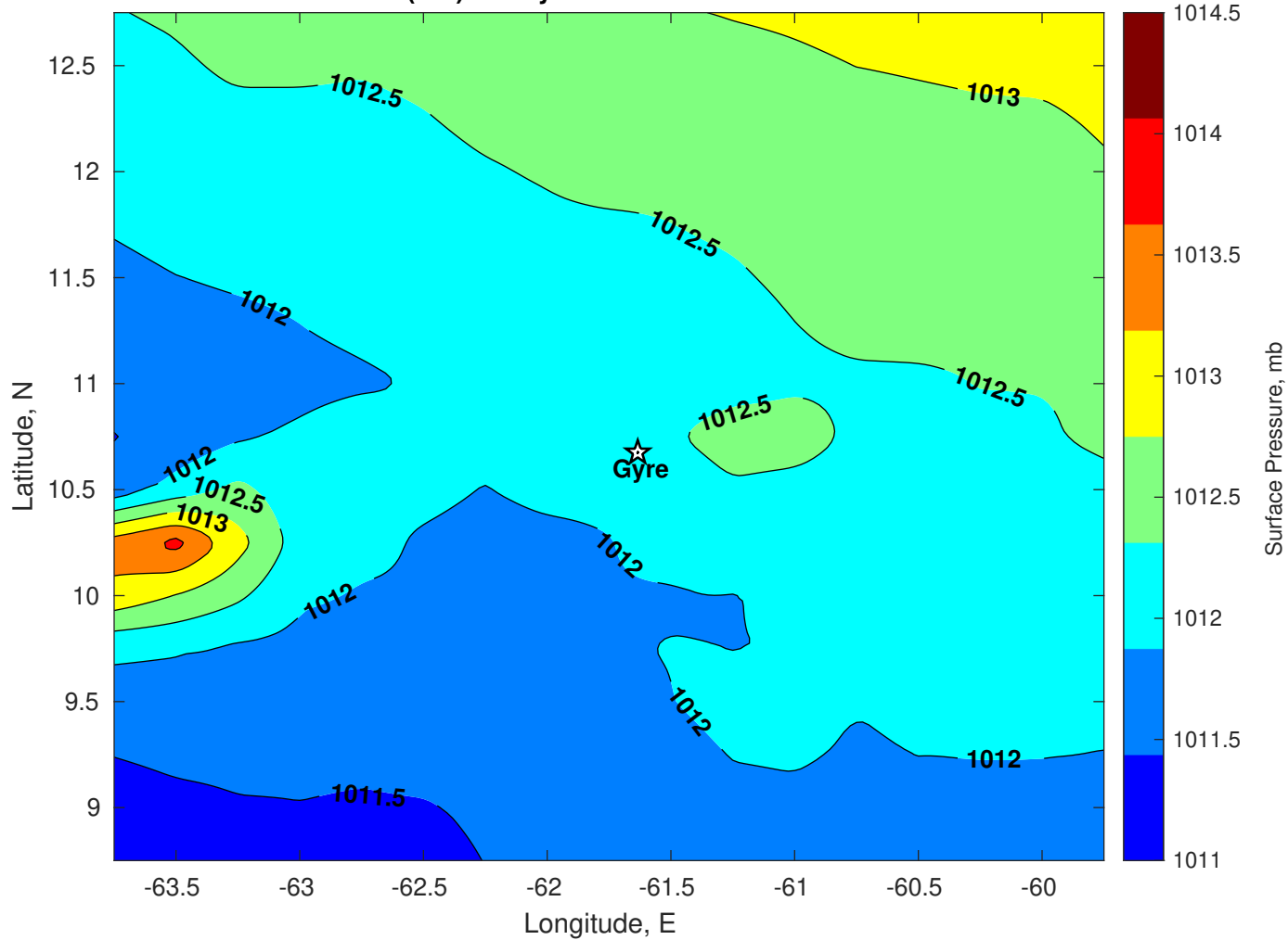
Surface Pressure (mb) for Gyre at 17-Dec-2025 00:00:00
