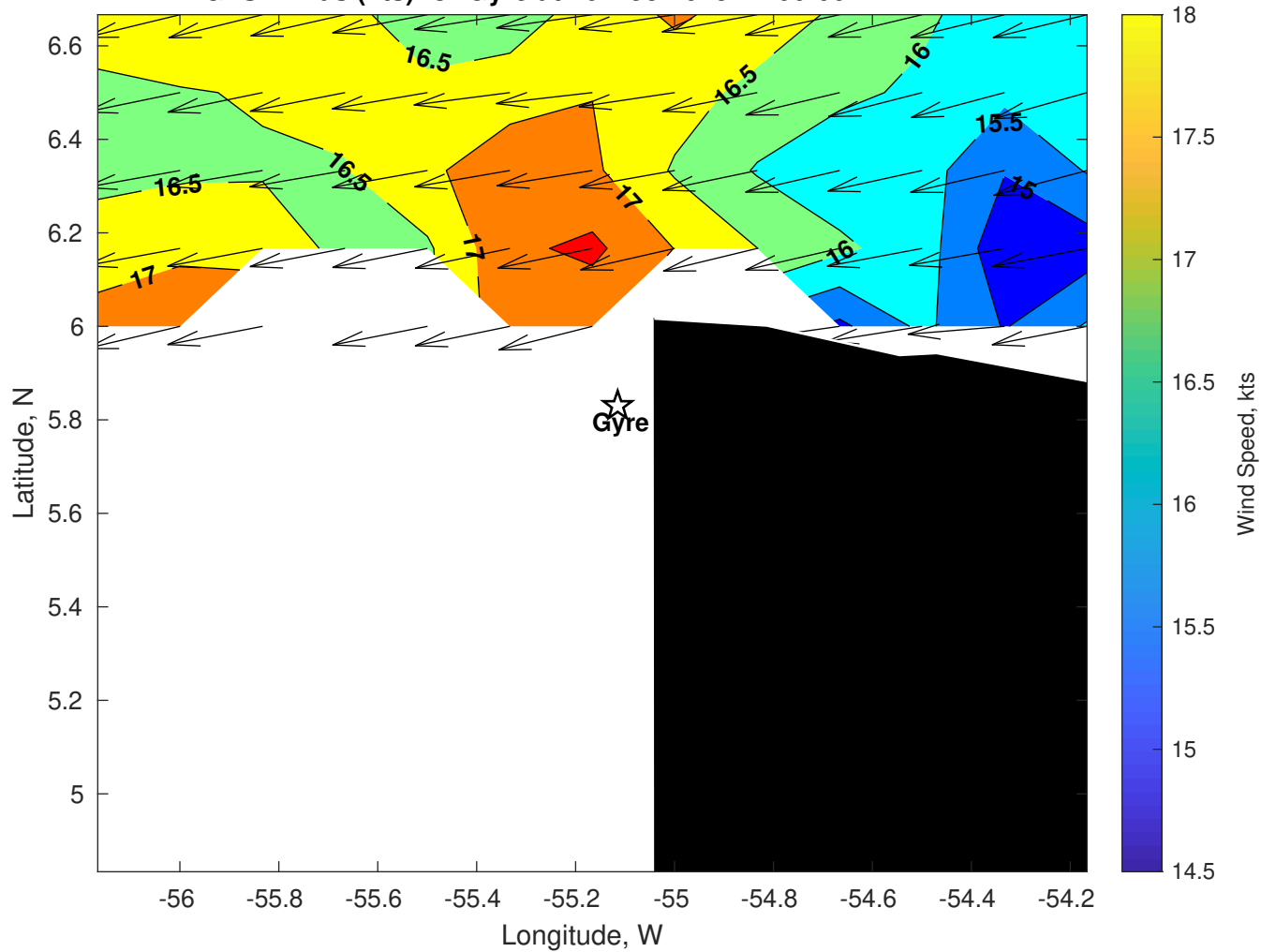
GFS Winds (kts) for Gyre at 10-Dec-2025 21:00:00
