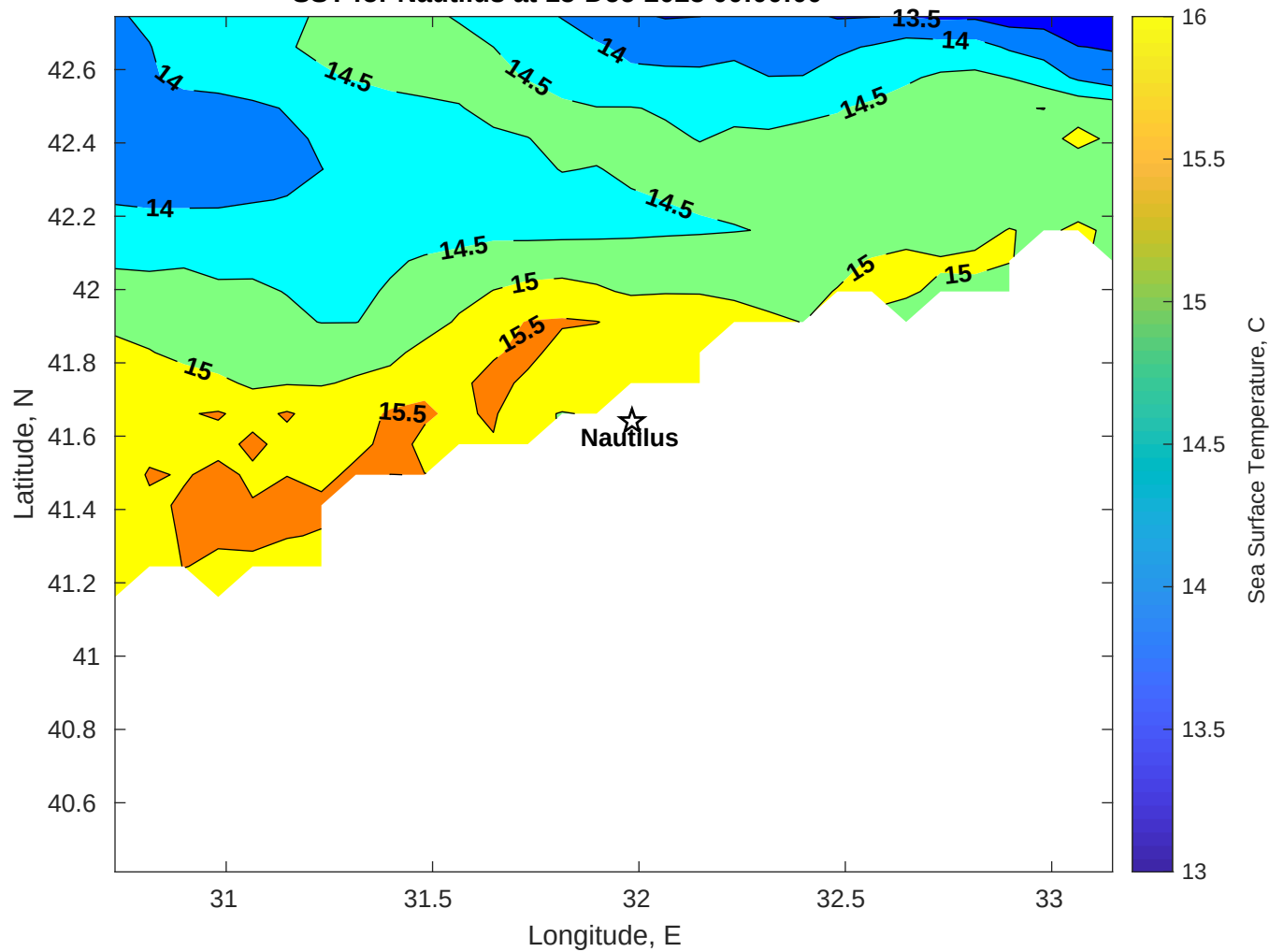
SST for Nautilus at 15-Dec-2025 00:00:00
