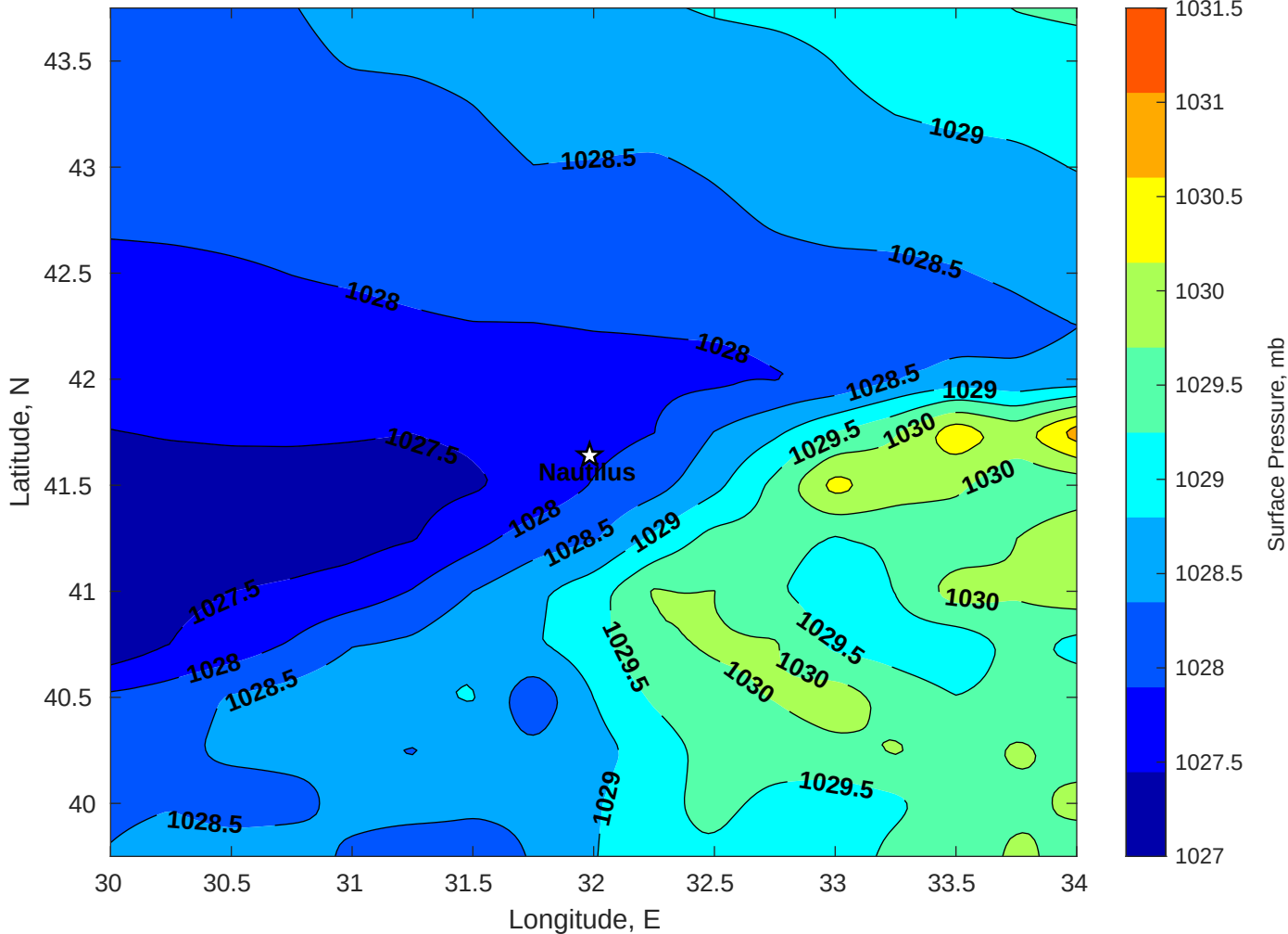
Surface Pressure (mb) for Nautilus at 17-Dec-2025 00:00:00
