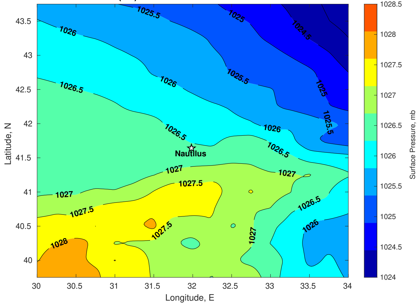
Surface Pressure (mb) for Nautilus at 16-Dec-2025 00:00:00
