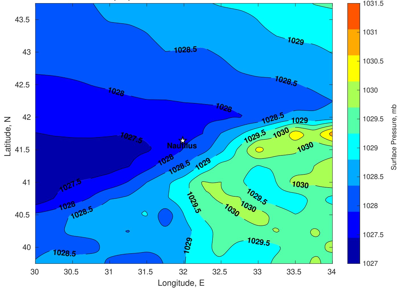
Surface Pressure (mb) for Nautilus at 17-Dec-2025 00:00:00
