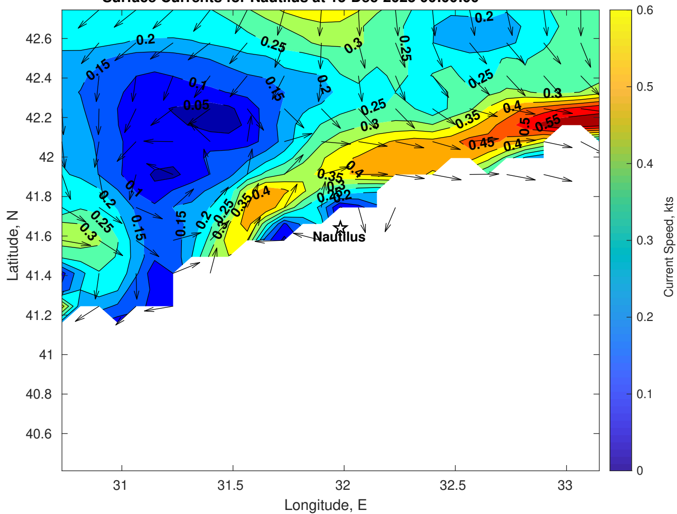
Surface Currents for Nautilus at 15-Dec-2025 00:00:00
