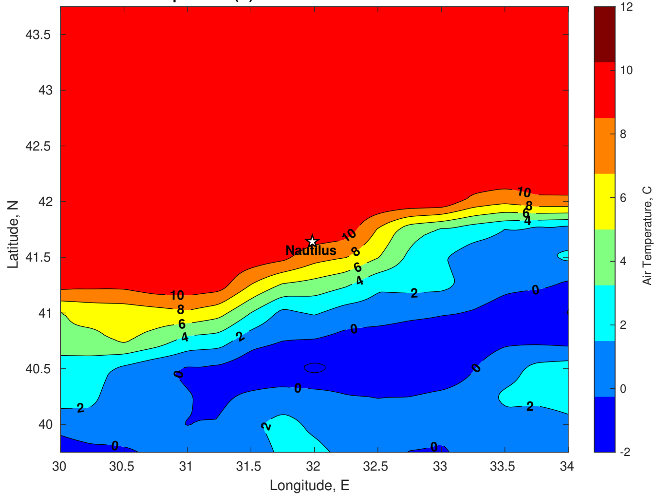
Air Temperature (C) for Nautilus at 16-Dec-2025
