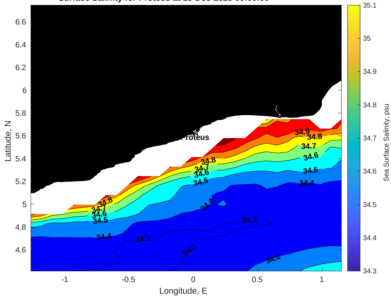
Surface Salinity for Proteus at 15-Dec-2025 00:00:00
