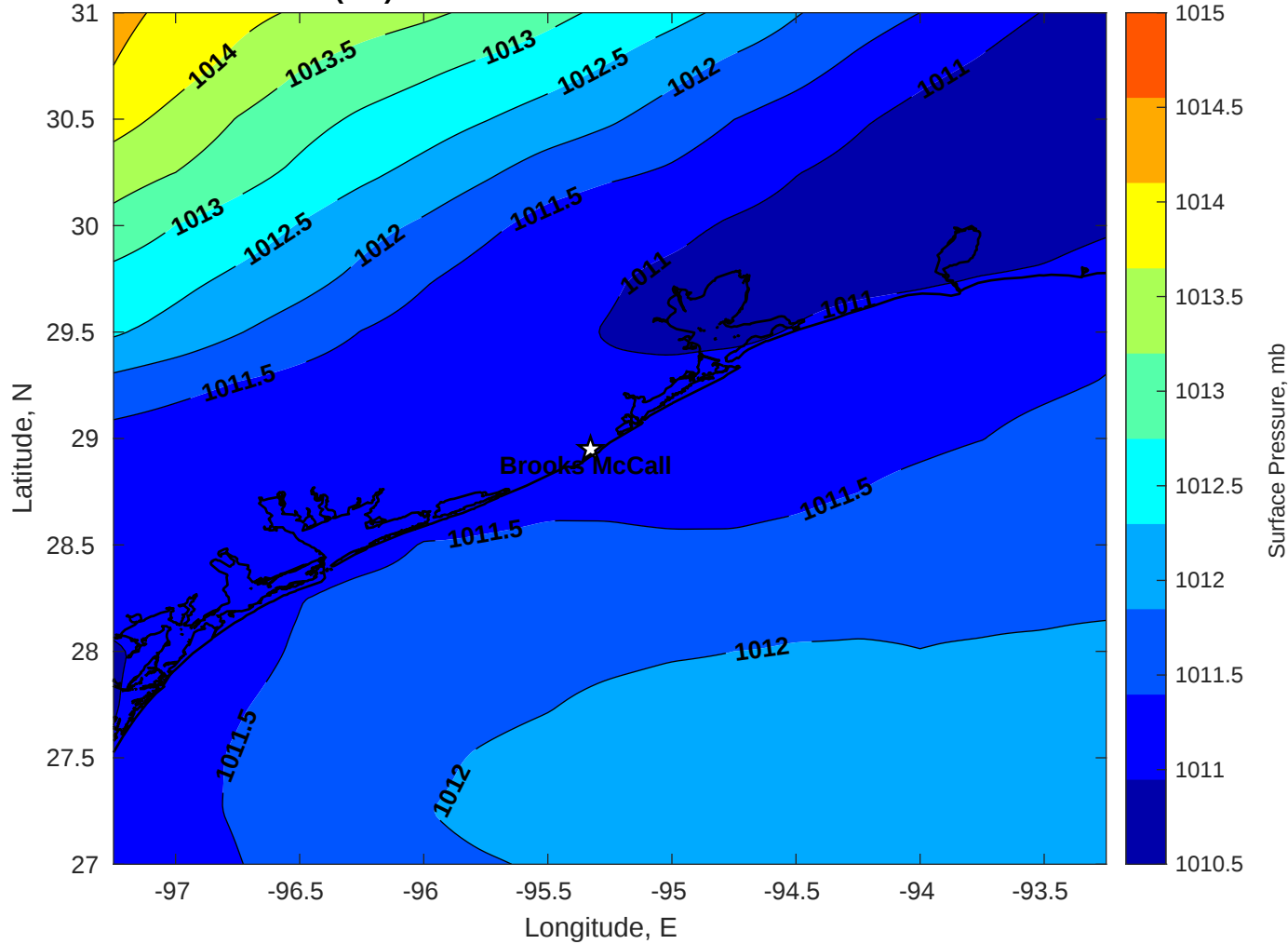
Surface Pressure (mb) for Brooks McCall at 19-Dec-2025 00:00:00
