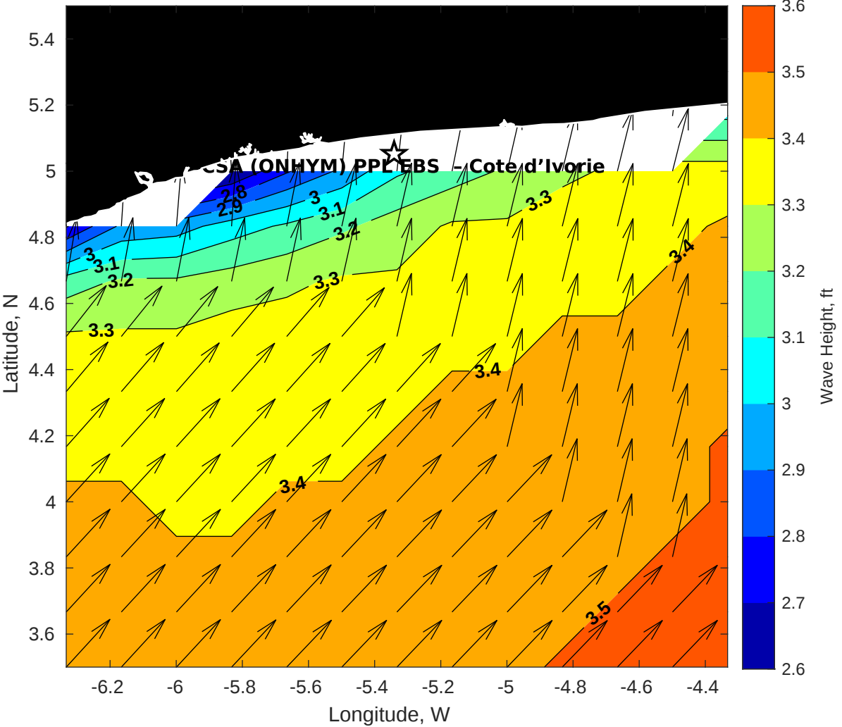
GFS Wave Height (ft) for CSA (ONHYM) PPL EBS - Cote d'Ivoire at 17-Dec-2025 09:00:00
