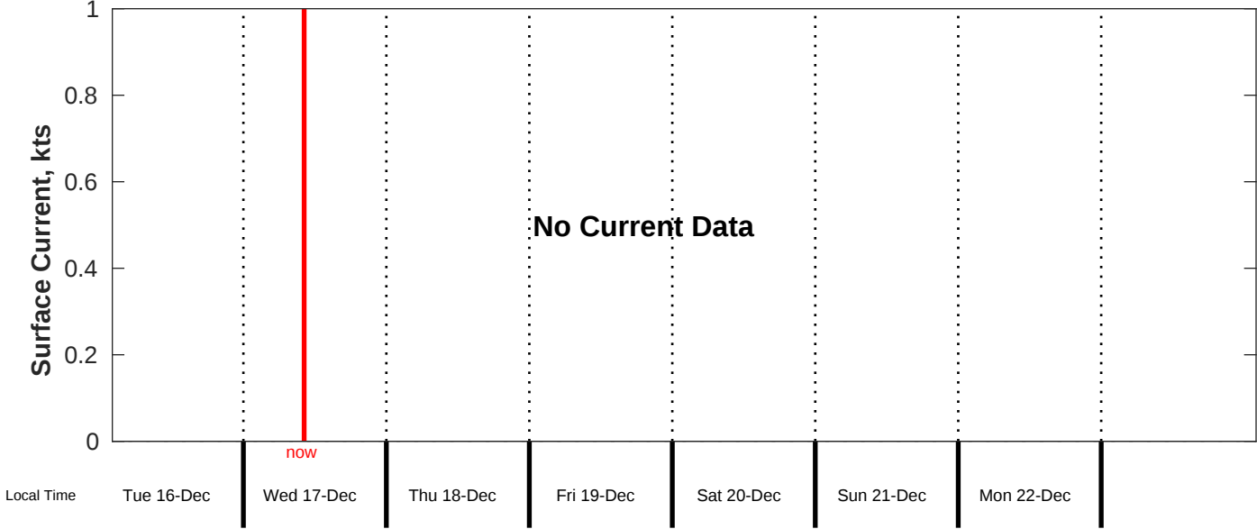
Surface Current Forecast for CSA (ONHYM) PPL EBS - Cote d'Ivoire from 16-Dec-2025 00:00:00 to 24-Dec-2025 00:00:00
