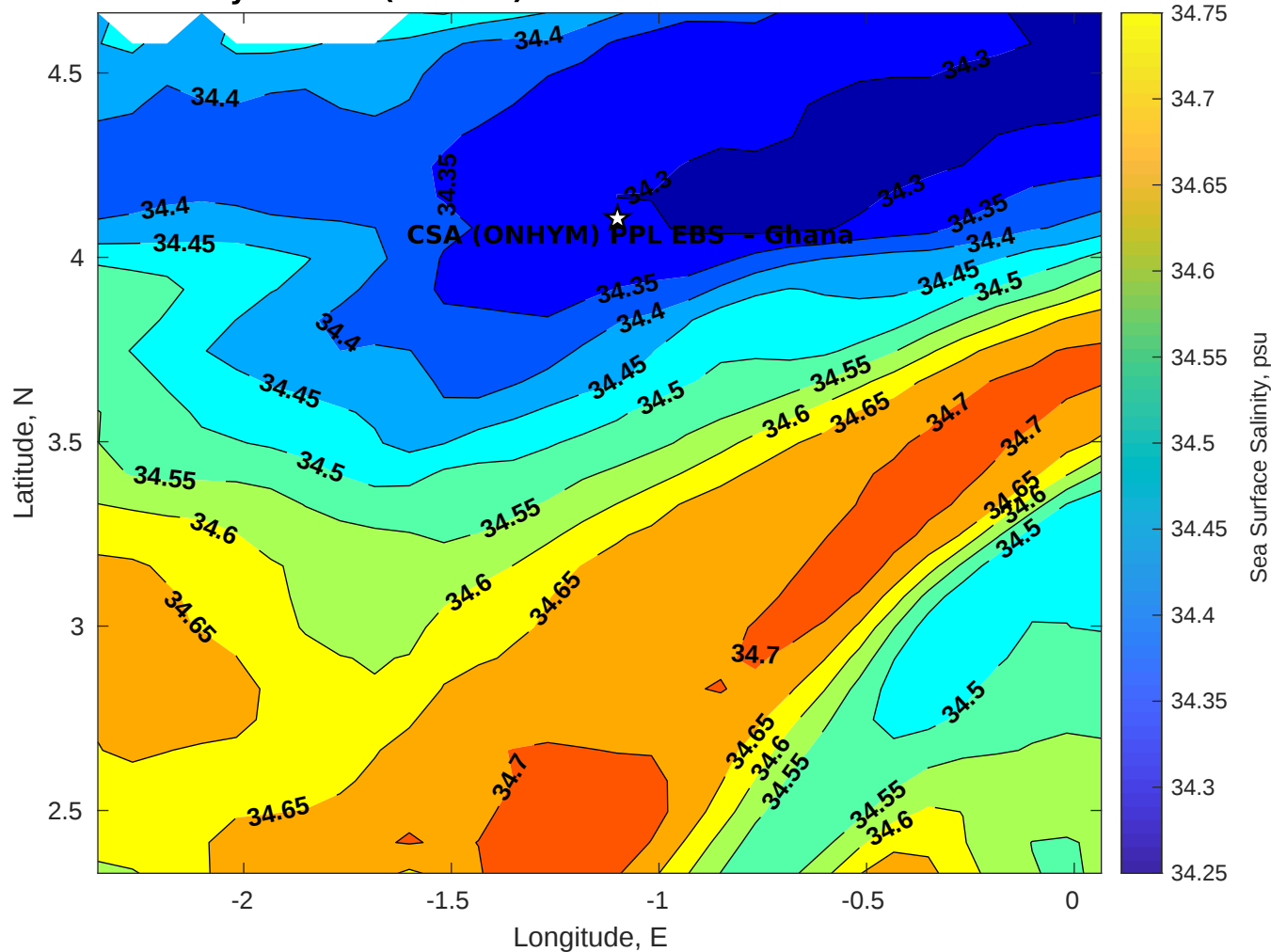
Surface Salinity for CSA (ONHYM) PPL EBS - Ghana at 16-Dec-2025 00:00:00
