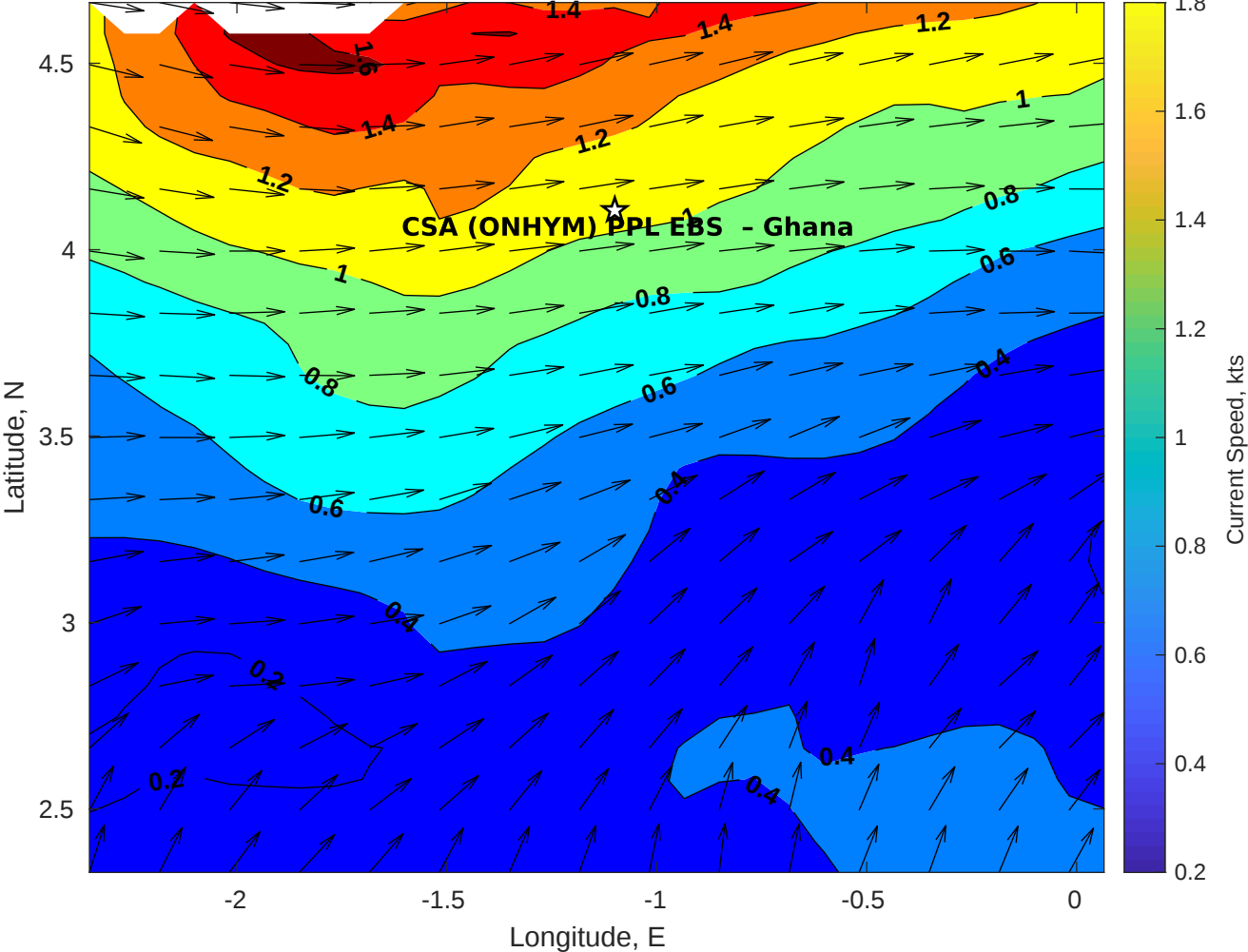
Surface Currents for CSA (ONHYM) PPL EBS - Ghana at 16-Dec-2025 00:00:00
