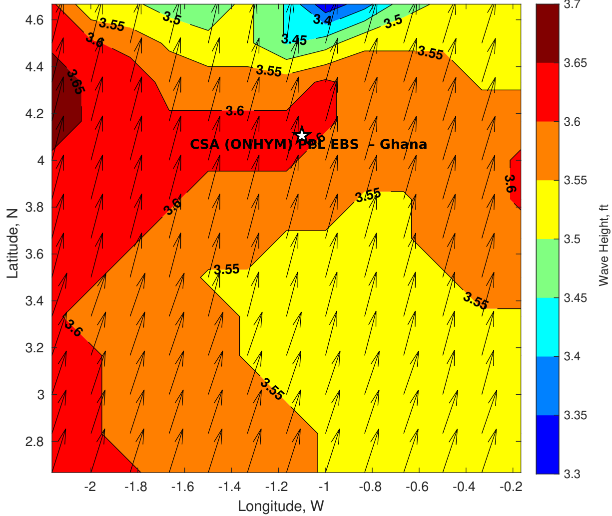
GFS Wave Height (ft) for CSA (ONHYM) PPL EBS - Ghana at 16-Dec-2025 21:00:00
