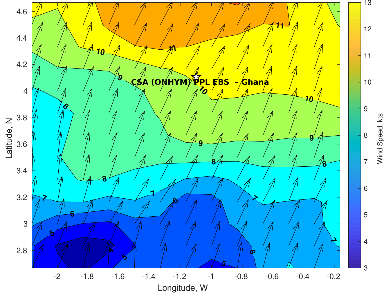
GFS Winds (kts) for CSA (ONHYM) PPL EBS - Ghana at 16-Dec-2025 21:00:00
