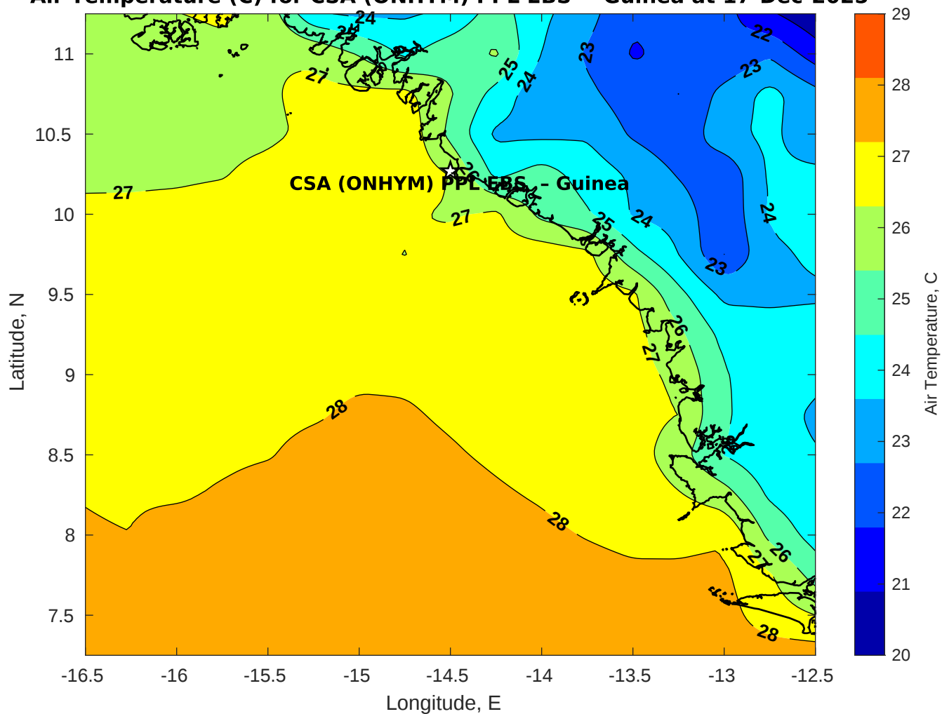
Air Temperature (C) for CSA (ONHYM) PPL EBS - Guinea at 17-Dec-2025
