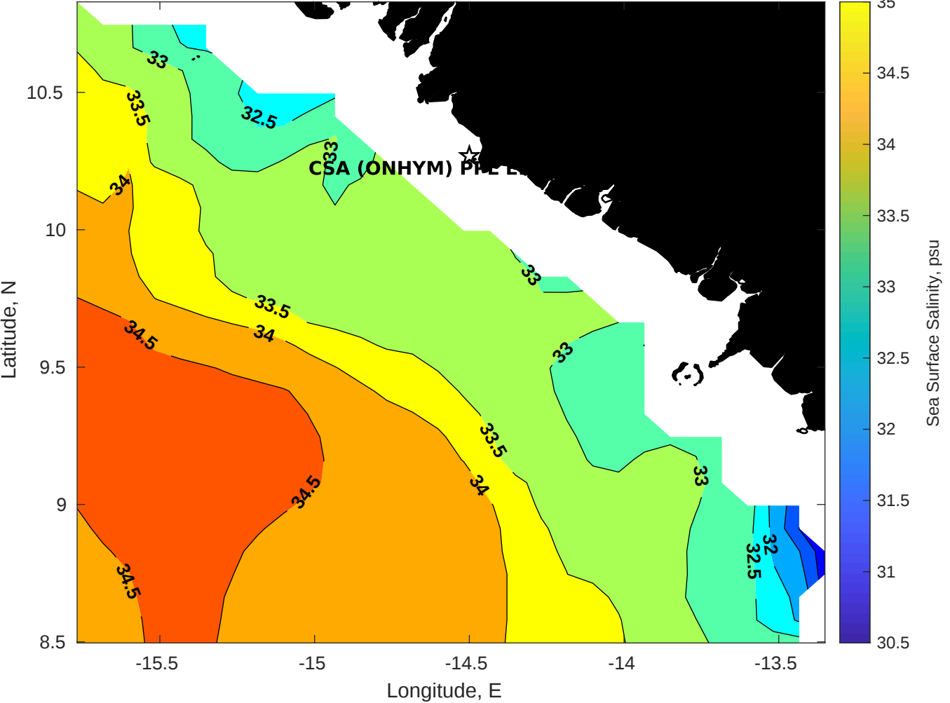
Surface Salinity for CSA (ONHYM) PPL EBS - Guinea at 16-Dec-2025 00:00:00
