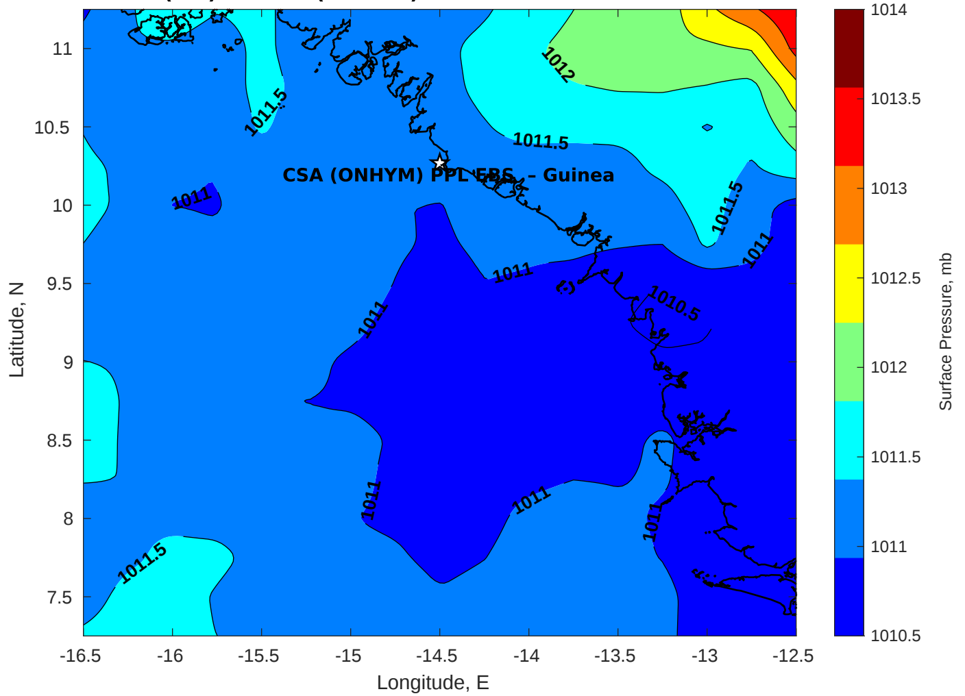
Surface Pressure (mb) for CSA (ONHYM) PPL EBS - Guinea at 18-Dec-2025 00:00:00
