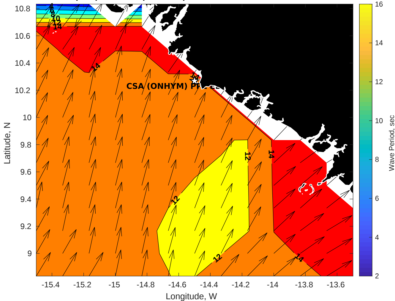
GFS Wave Period (sec) for CSA (ONHYM) PPL EBS - Guinea at 17-Dec-2025 09:00:00
