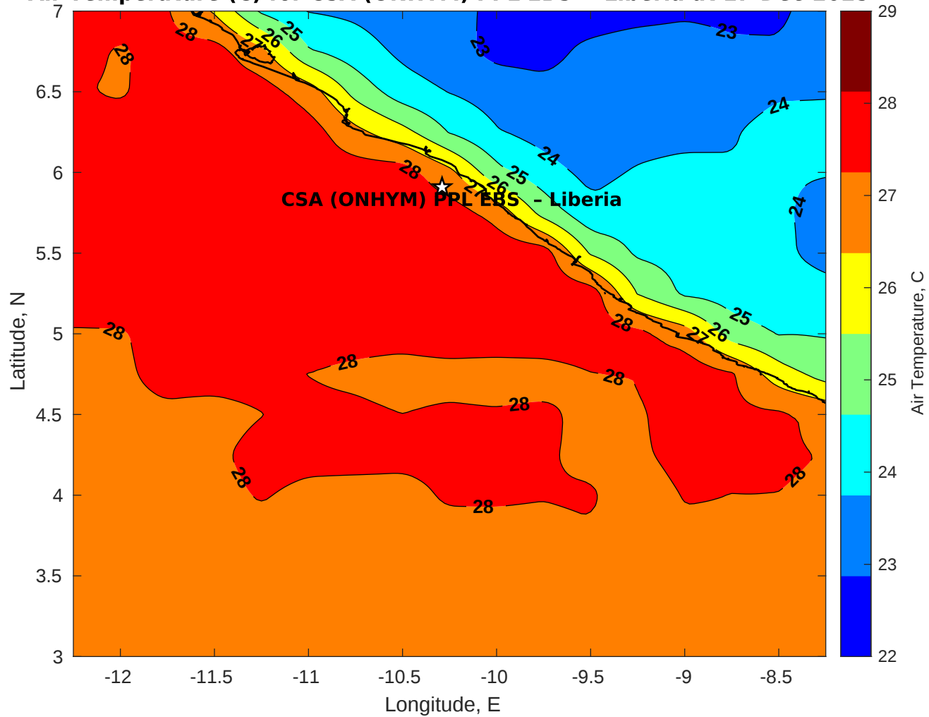
Air Temperature (C) for CSA (ONHYM) PPL EBS - Liberia at 17-Dec-2025
