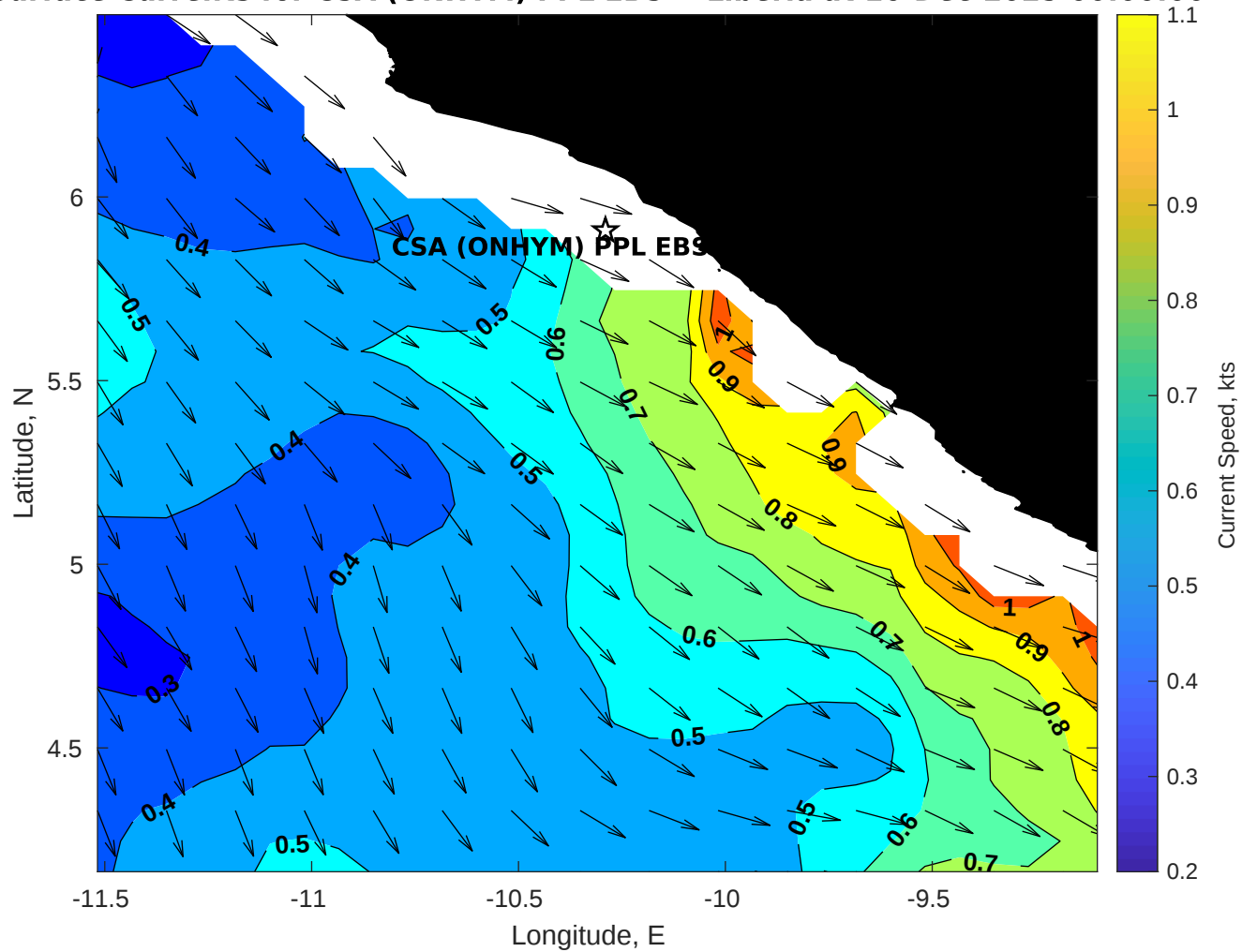
Surface Currents for CSA (ONHYM) PPL EBS - Liberia at 16-Dec-2025 00:00:00
