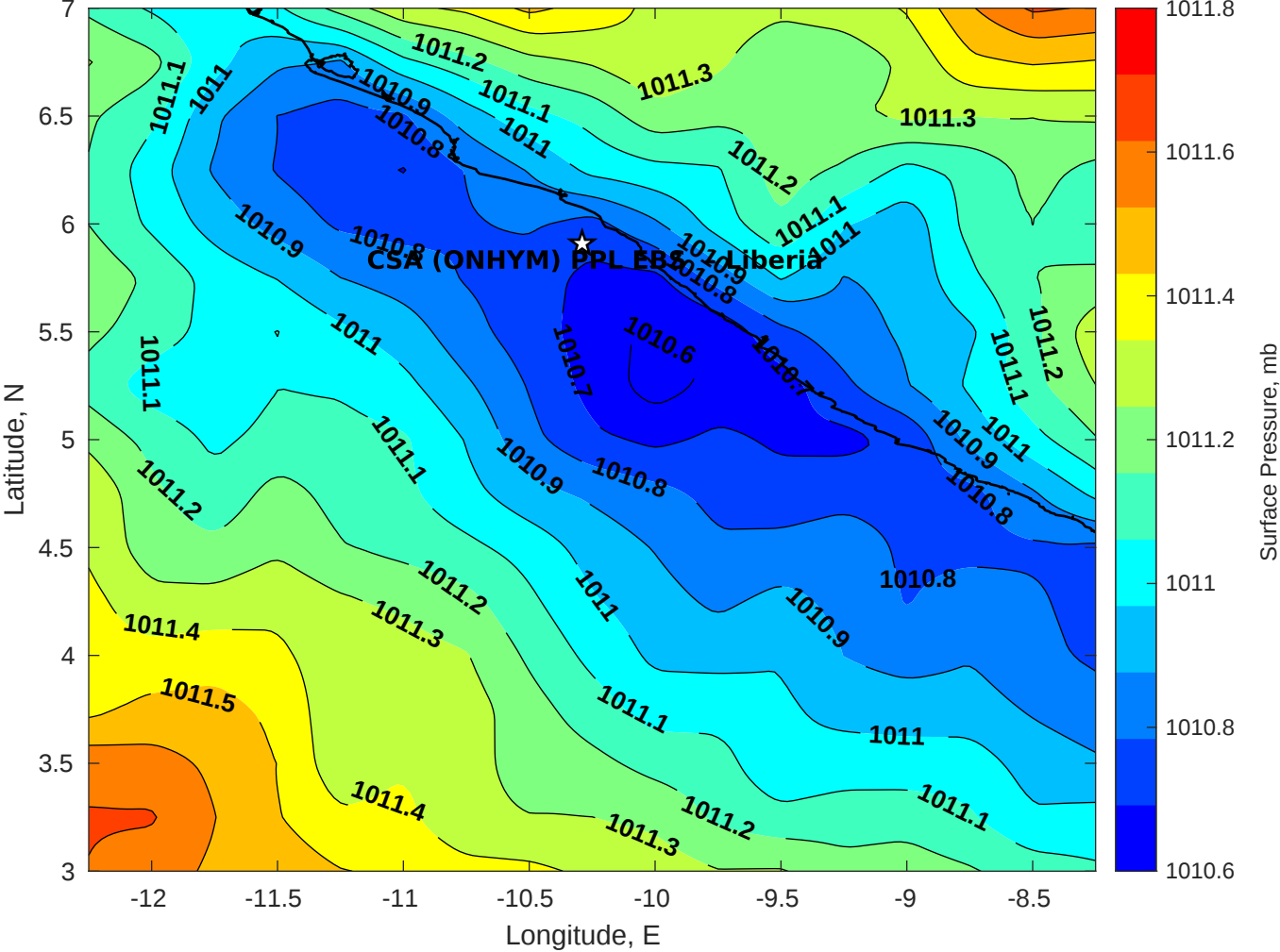
Surface Pressure (mb) for CSA (ONHYM) PPL EBS - Liberia at 17-Dec-2025 00:00:00
