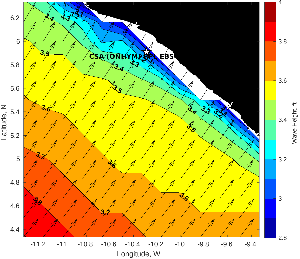
GFS Wave Height (ft) for CSA (ONHYM) PPL EBS - Liberia at 17-Dec-2025 09:00:00
