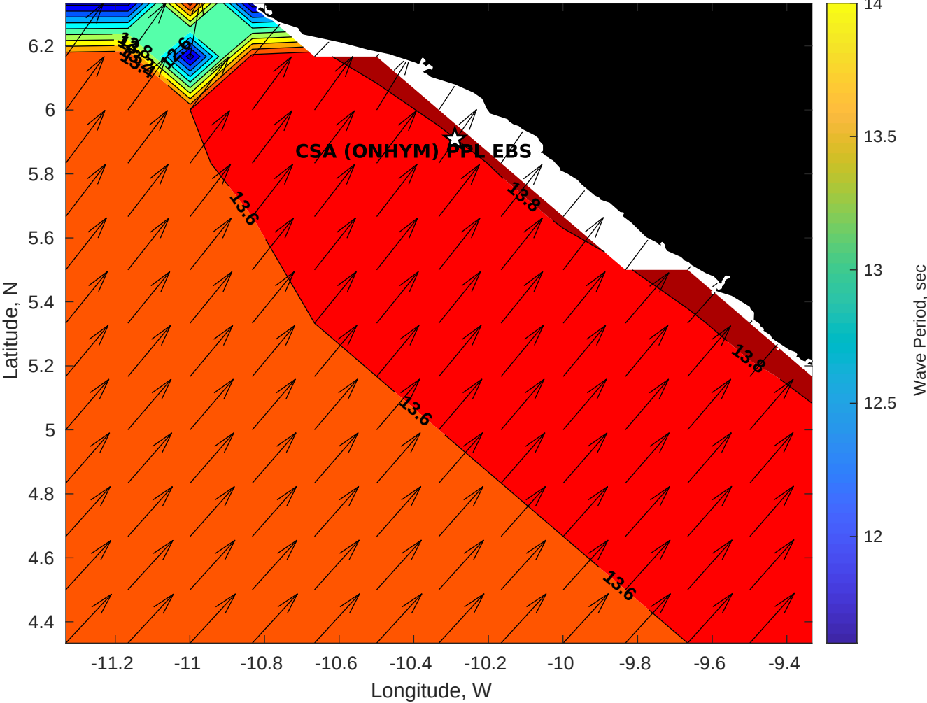
GFS Wave Period (sec) for CSA (ONHYM) PPL EBS - Liberia at 17-Dec-2025 09:00:00
